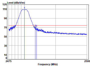
PIFA ANT BLE_2M_TX_CH_39_Vertical-Peak
