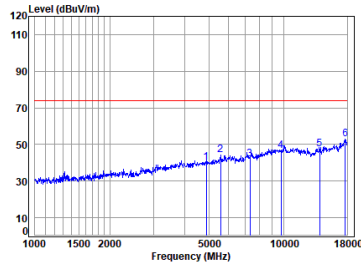
FPC ANT BLE_2M_TX_CH_19_Vertical-Peak
