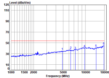
PIFA ANT BLE_2M_TX_CH_19_Vertical-Avg
