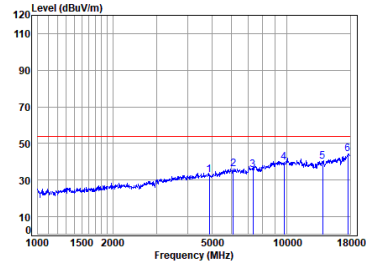
FPC ANT BLE_2M_TX_CH_19_Horizontal-Avg
