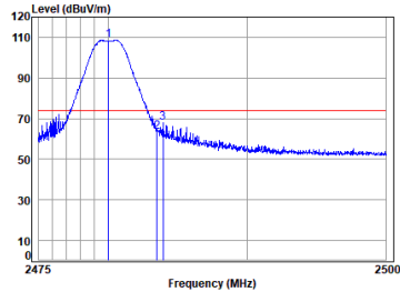
PIFA ANT BLE_2M_TX_CH_39_Horizontal-Peak
