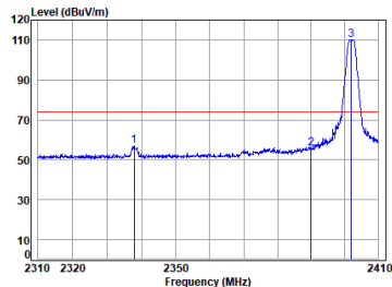
FPC ANT BLE_2M_TX_CH_00_Vertical-Peak
