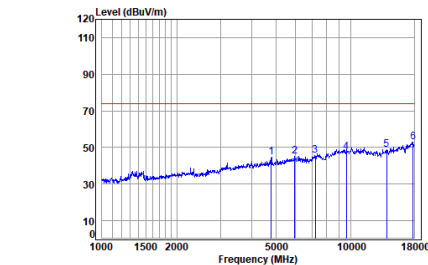
PIFA ANT BLE_2M_TX_CH_00_Vertical-Peak
