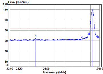
FPC ANT BLE_2M_TX_CH_00_Horizontal-Peak
