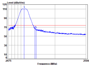
FPC ANT BLE_2M_TX_CH_39_Vertical-Peak
