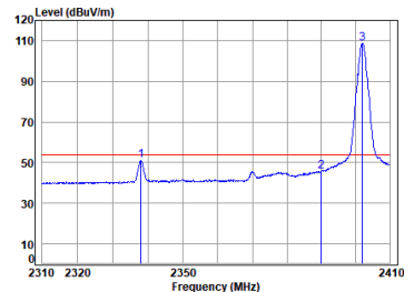
FPC ANT BLE_2M_TX_CH_00_Vertical-Avg
