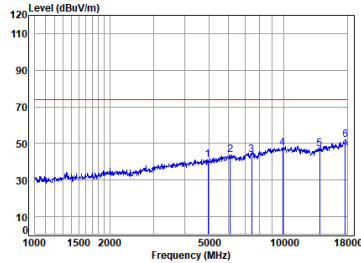
FPC ANT BLE_2M_TX_CH_39_Horizontal-Peak
