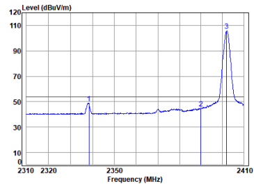
PIFA ANT BLE_2M_TX_CH_00_Horizontal-Avg
