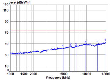
PIFA ANT BLE_2M_TX_CH_19_Horizontal-Peak
