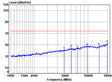
FPC ANT BLE_2M_TX_CH_19_Horizontal-Peak
