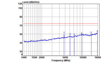
PIFA ANT BLE_2M_TX_CH_00_Horizontal-Peak
