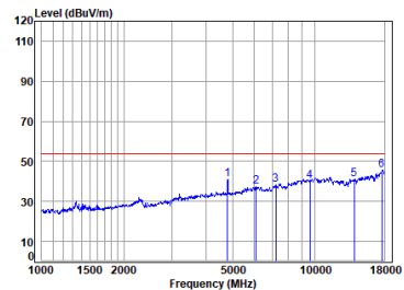
PIFA ANT BLE_2M_TX_CH_00_Vertical-Avg
