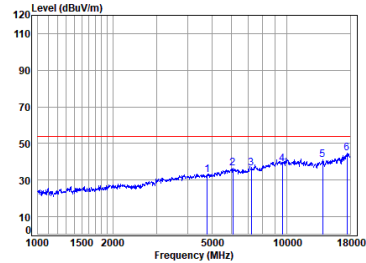
FPC ANT BLE_2M_TX_CH_00_Horizontal-Avg
