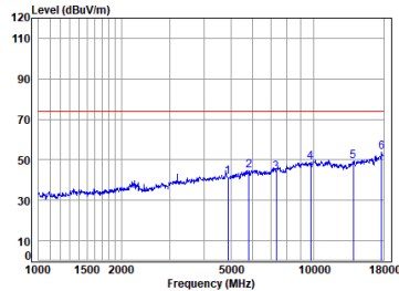
PIFA ANT BLE_2M_TX_CH_19_Vertical-Peak
