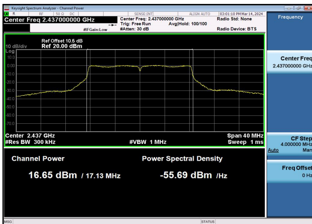
Output Power-802.11g,2437MHz,Ant0
