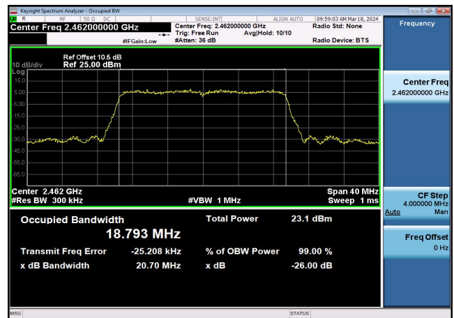
99% Bandwidth-802.11ax(20MHz),2462MHz ,Ant0
