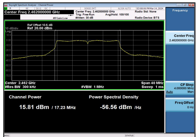
Output Power-802.11g,2462MHz,Ant0
