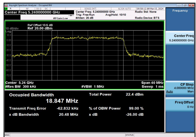
U-NII-1 99%&26dB Bandwidth-802.11ax(20MHz) ,5240MHz,Ant1
