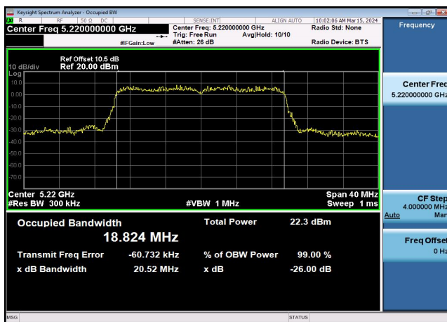
U-NII-1 99%&26dB Bandwidth-802.11ax(20MHz) ,5220MHz,Ant1
