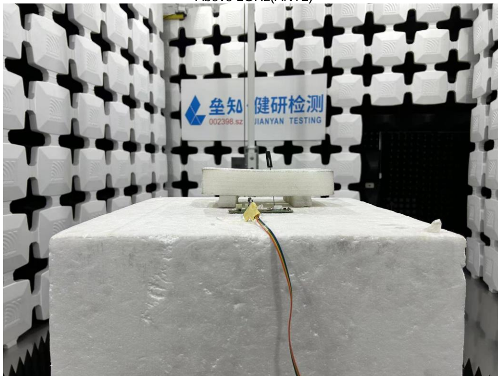
Radiated Spurious Emission Above 1GHz(ANT2)
