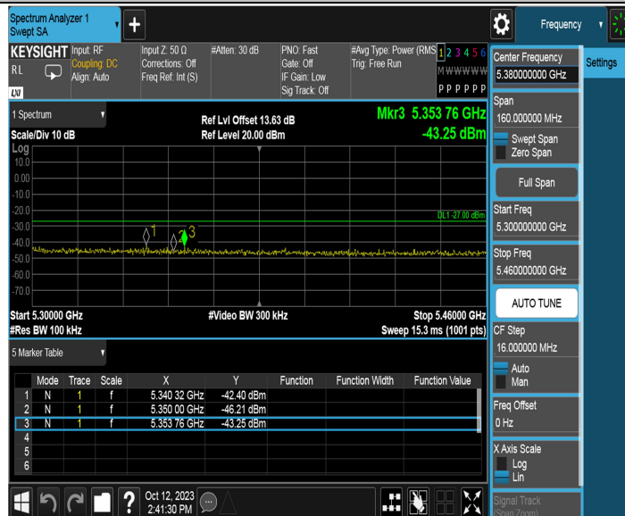
11N40MIMO_Ant2_High_5310
