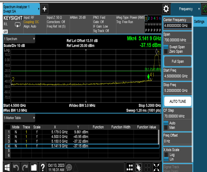
11AC20MIMO_Ant1_Low_5180_Peak
