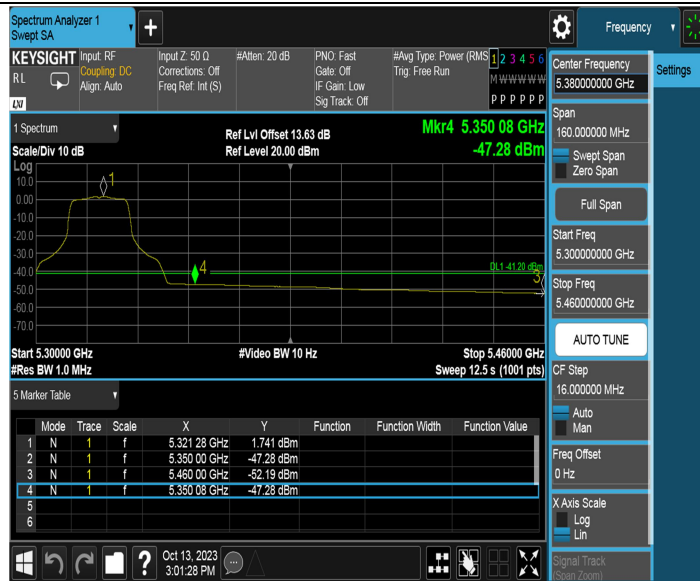
11AC20MIMO_Ant1_High_5320_Peak
