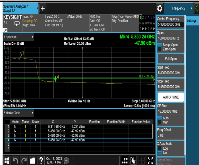
11AC40MIMO_Ant1_High_5310_Peak
