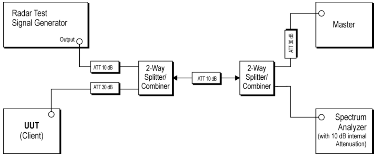
Figure 3-1: Conducted Setup
