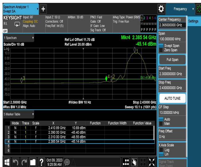
11B_Ant2_Low_2412_Peak
