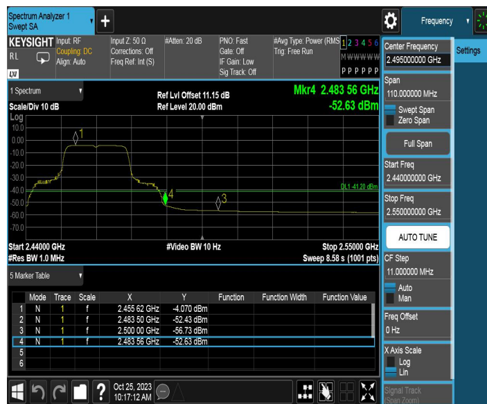
11AX20MIMO_Ant1_High_2462_Peak
