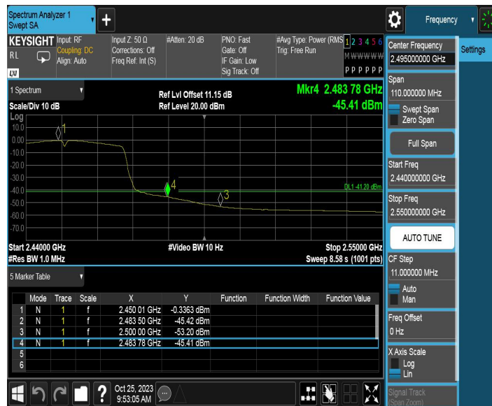
11N40MIMO_Ant1_High_2452_Peak
