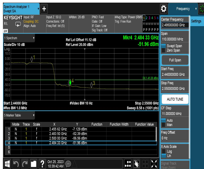
11AX40MIMO_Ant2_High_2452_Peak
