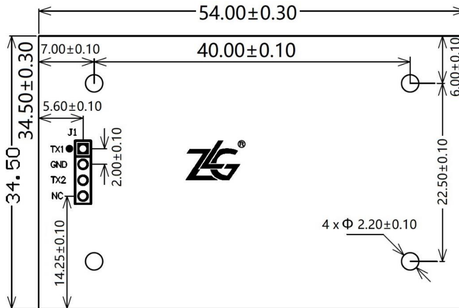
Figure 4 ZLG600A-ANT Dimension
