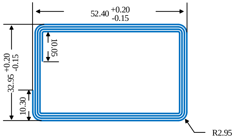
Figure 5 ZLG600A PCB Antenna Dimension
