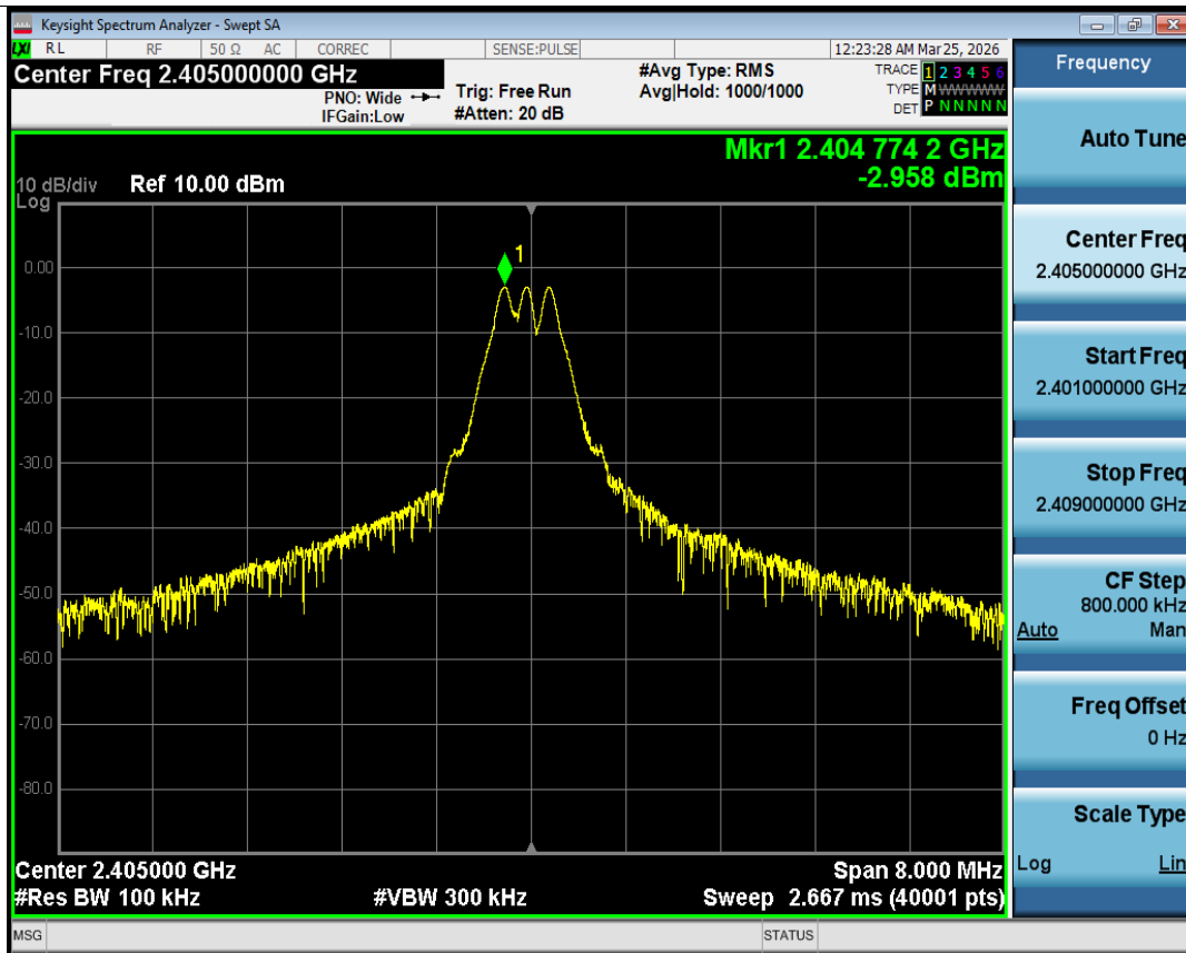
Tx. Spurious NVNT 2.4G 2405MHz Ant1 Ref
