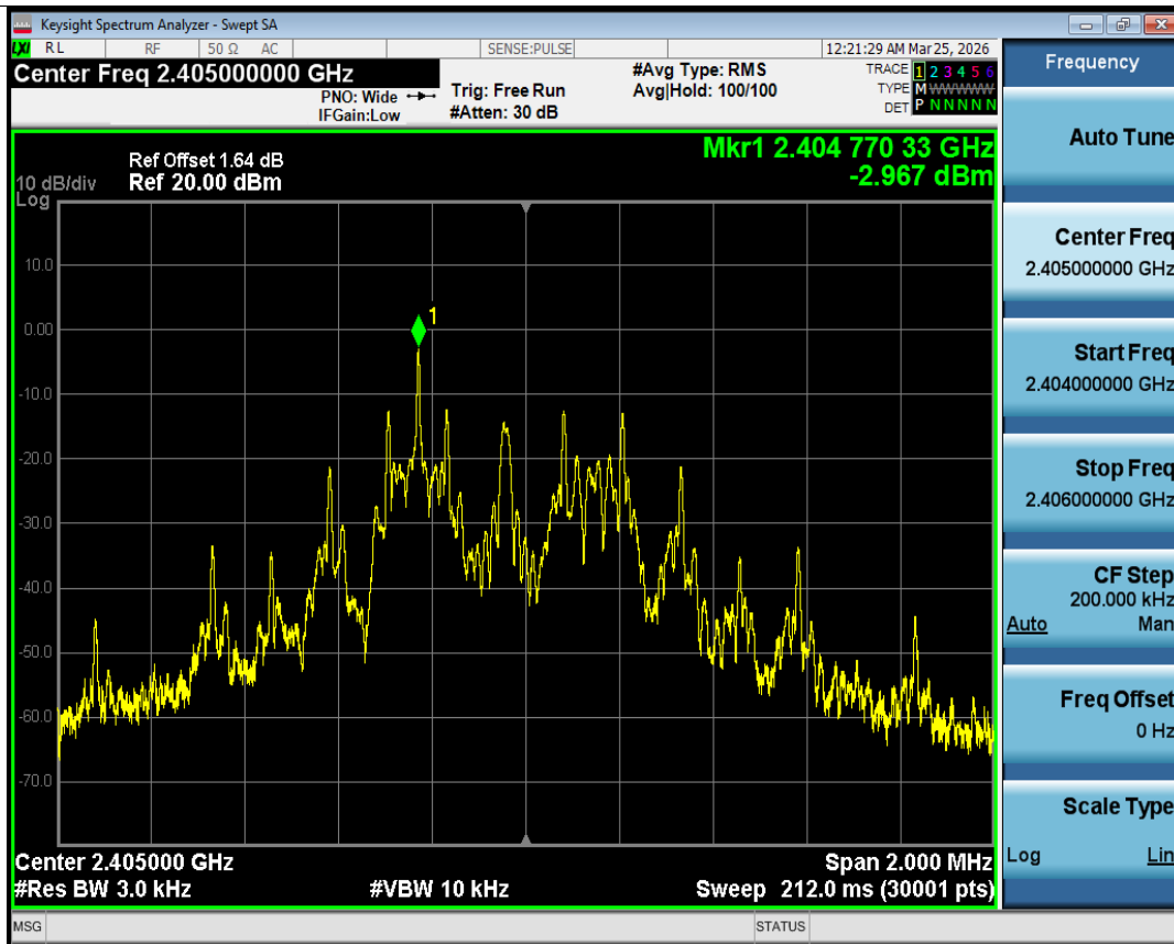
PSD NVNT 2.4G 2405MHz Ant1
