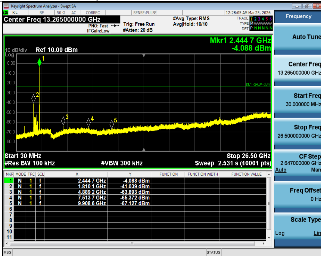
Tx. Spurious NVNT 2.4G 2445MHz Ant1 Emission
