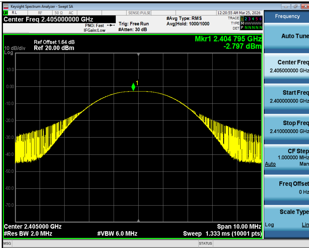
Peak Power NVNT 2.4G 2405MHz Ant1
