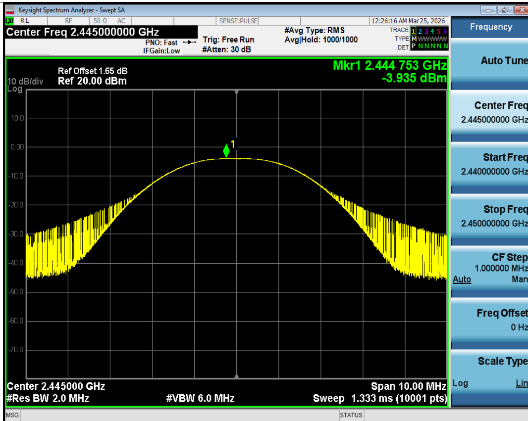
Peak Power NVNT 2.4G 2445MHz Ant1
