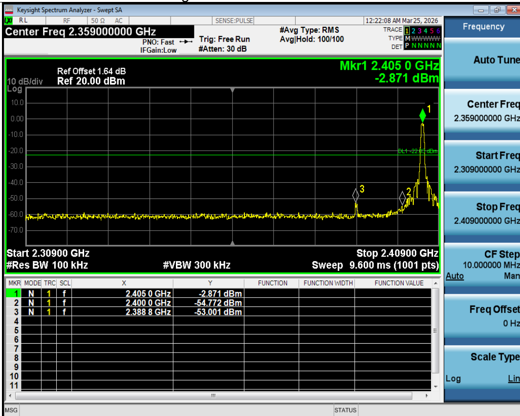
Band Edge NVNT 2.4G 2405MHz Ant1 Emission
