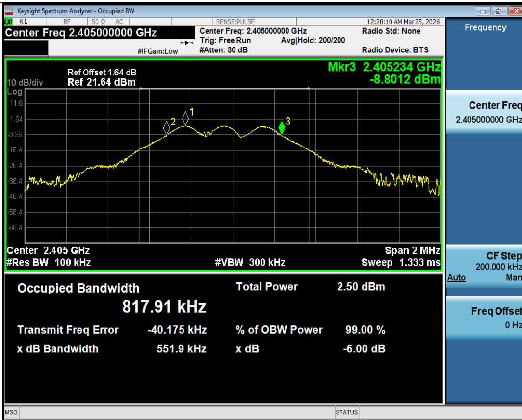
-6dB Bandwidth NVNT 2.4G 2405MHz Ant1
