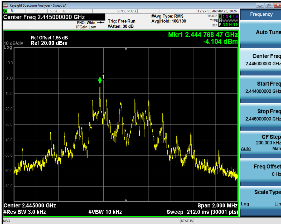
PSD NVNT 2.4G 2445MHz Ant1
