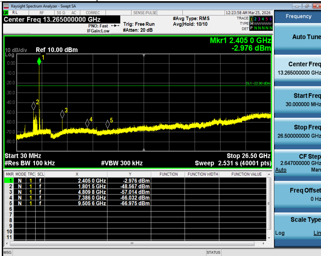
Tx. Spurious NVNT 2.4G 2405MHz Ant1 Emission
