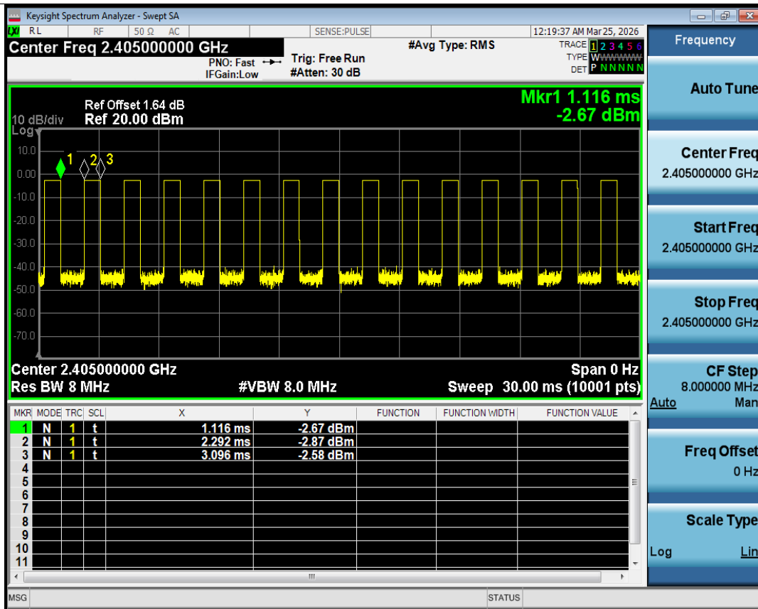
Duty Cycle NVNT 2.4G 2405MHz Ant1
