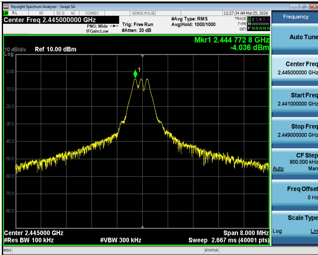
Tx. Spurious NVNT 2.4G 2445MHz Ant1 Ref
