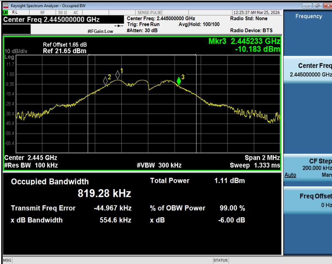
-6dB Bandwidth NVNT 2.4G 2445MHz Ant1
