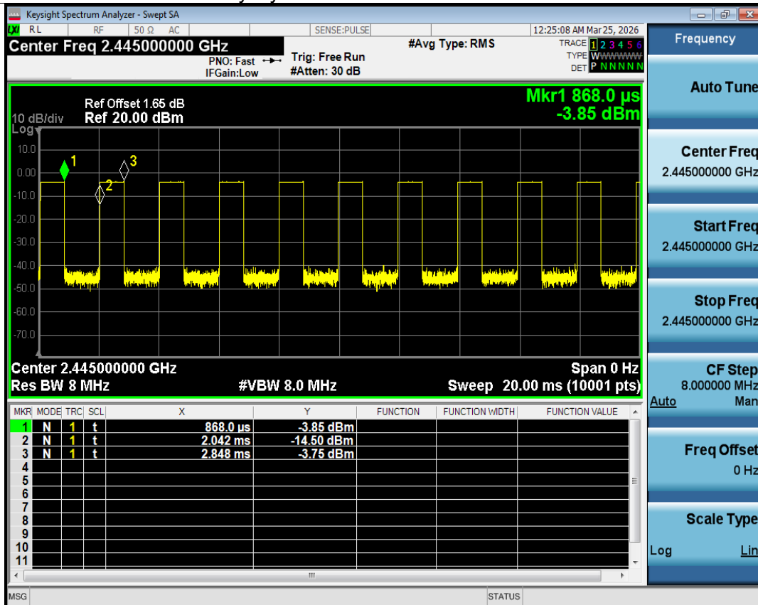
Duty Cycle NVNT 2.4G 2445MHz Ant1
