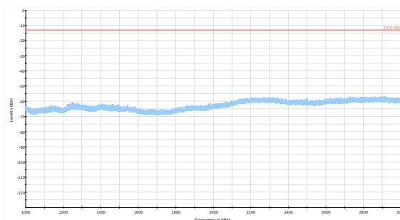
LTE Band 5 (1.4M) RB1 Middle Channel Link Mode 1GHz -3GHz
