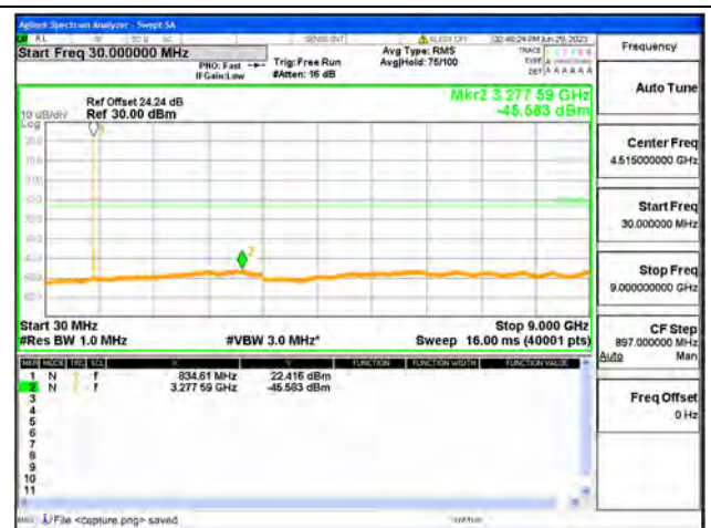
Band26 Part22 / 5MHz / Mid CH / QPSK
