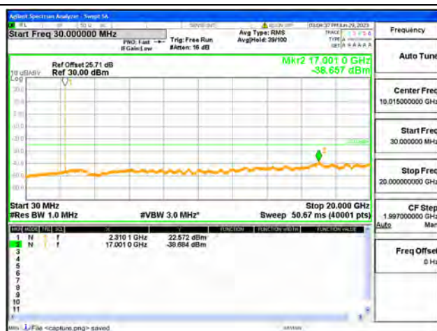
Band30-Band30M-20G / 5MHz / High CH / QPSK
