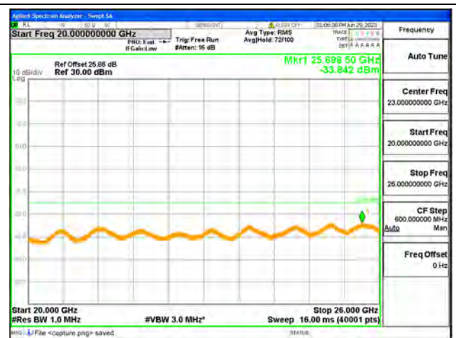
Band7-20G-26G / 5MHz / Low CH / QPSK
