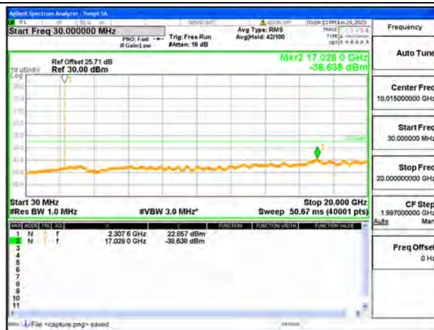
Band30-Band30M-20G / 5MHz / Mid CH / QPSK
