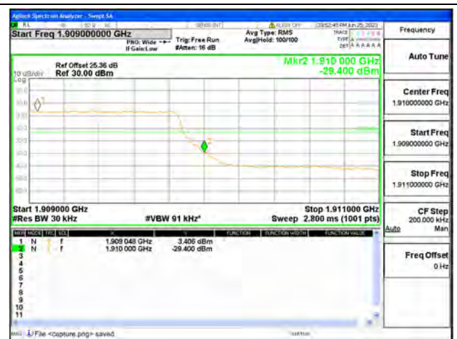
Band2 / 3MHz / High CH / QPSK / FULL RB
