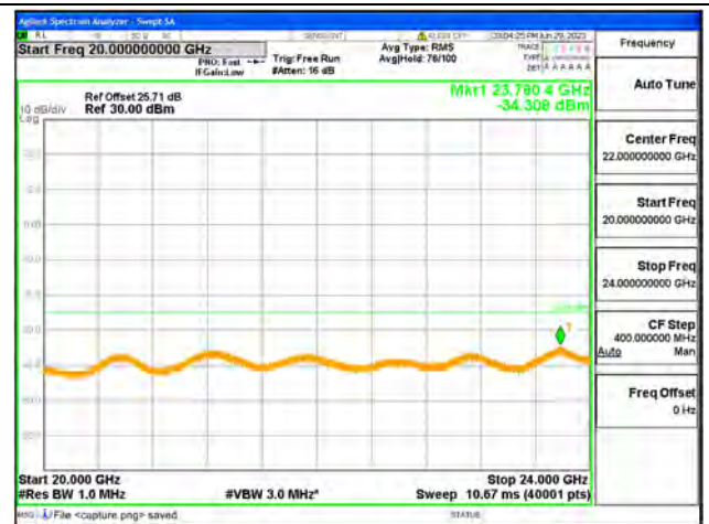
Band30-20G-24G / 5MHz / Mid CH / QPSK
