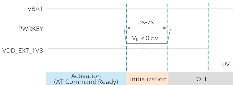
Figure 12. Power-off Sequence
