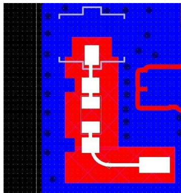
Figure 28. RF Traces
