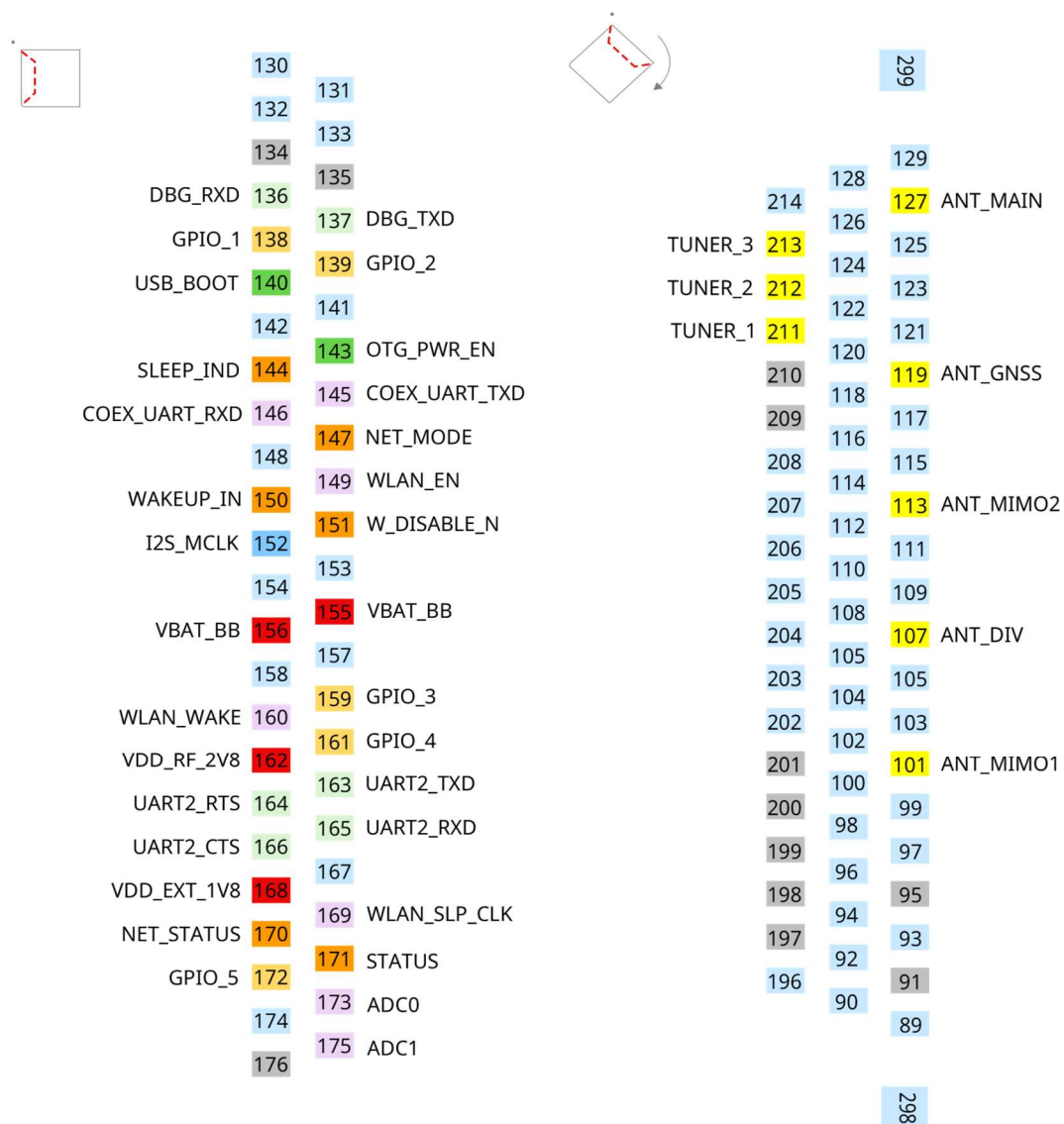
Figure 3. Pin Details (1)
