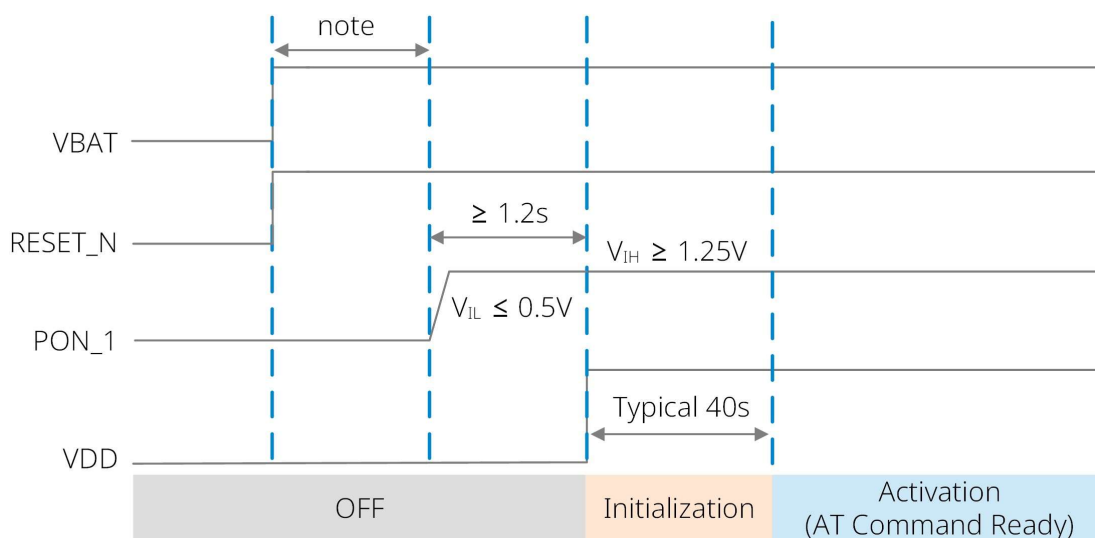
Figure 10. Power-on Sequence (PWRKEY)
