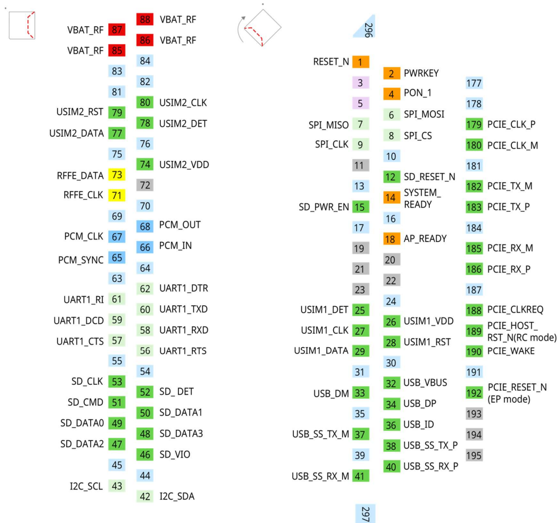
Figure 4. Pin Details (2)
