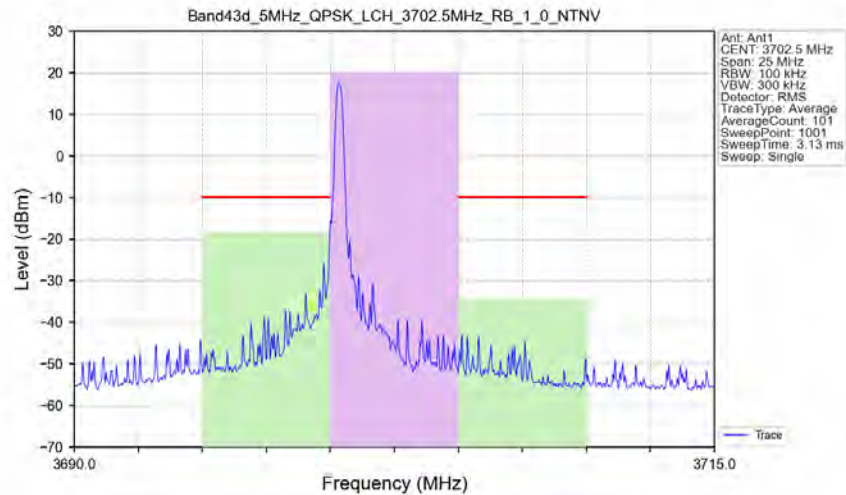
Band43d 5MHz QPSK LCH 3702.5MHz RB 1 0 NTNV
