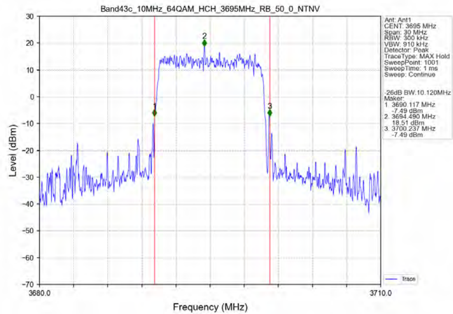
Band43c_10MHz_64QAM_HCH_3695MHz_RB_50_0_NTNV
