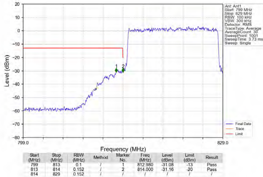
Band26c_15MHz_QPSK_LCH_821.5MHz_RB_75_0_NTNV
