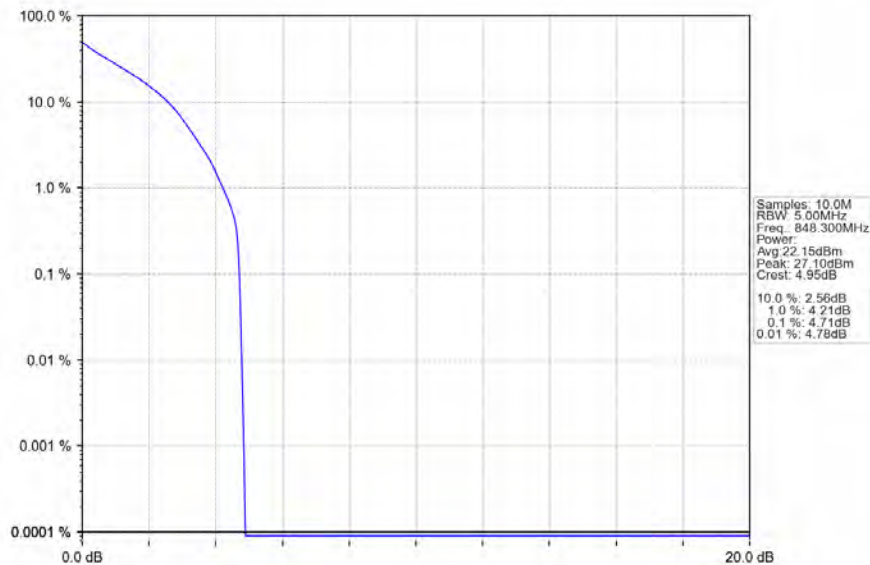
Band26b_1.4MHz_QPSK_HCH_848.3MHz_RB_6_0_NTNV
