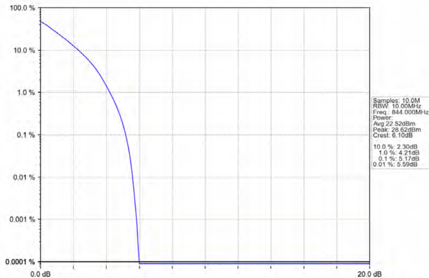
Band26b_10MHz_QPSK_HCH_844MHz_RB_50_0_NTNV
