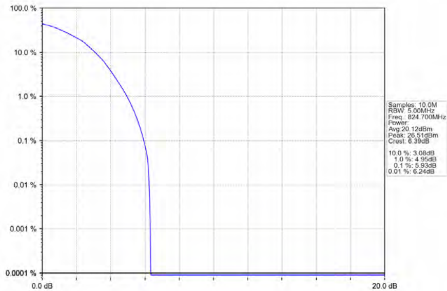
Band26b_1.4MHz_64QAM_LCH_824.7MHz_RB_6_0_NTNV
