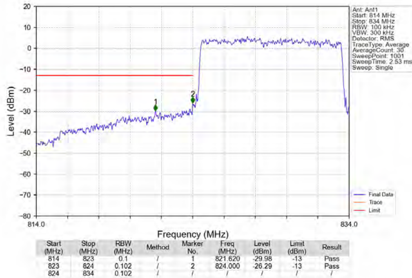
Band26b_10MHz_QPSK_LCH_829MHz_RB_50_0_NTNV
