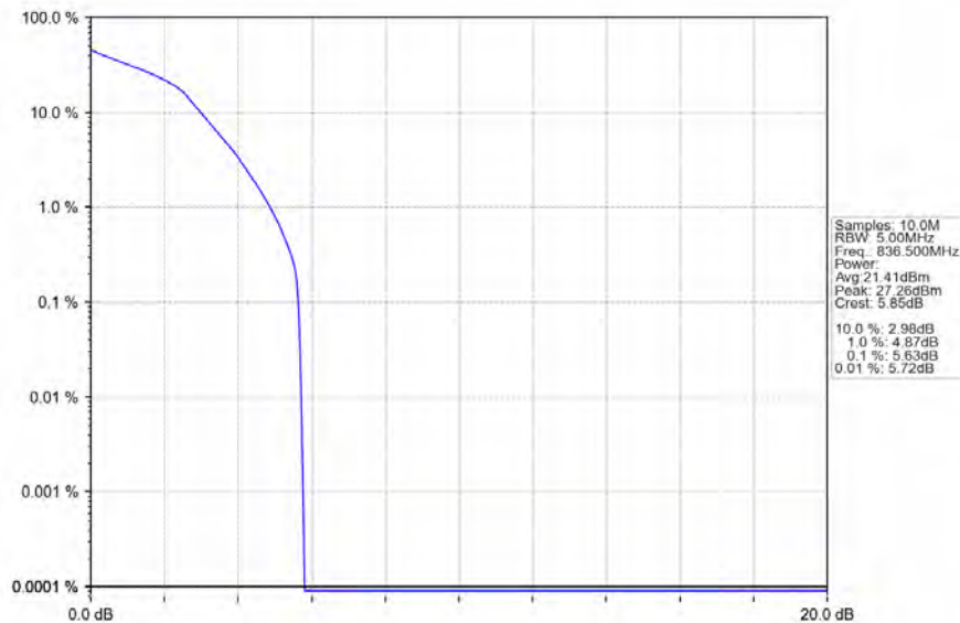
Band26b_1.4MHz_16QAM_MCH_836.5MHz_RB_6_0_NTNV
