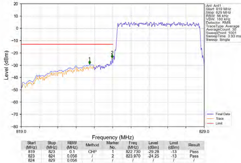
Band26b_5MHz_QPSK_LCH_826.5MHz_RB_25_0_NTNV
