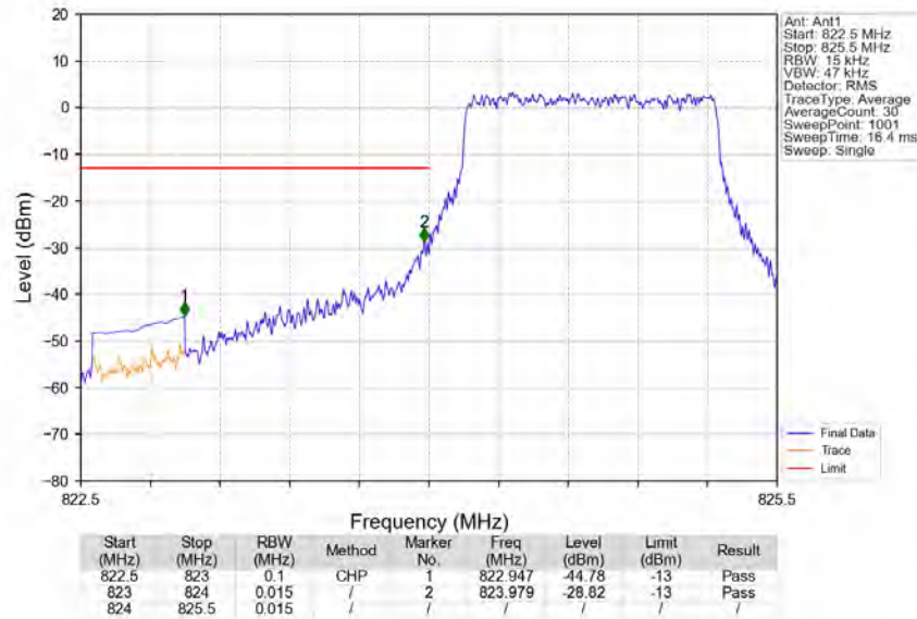
Band26b_1.4MHz_64QAM_LCH_824.7MHz_RB_6_0_NTNV
