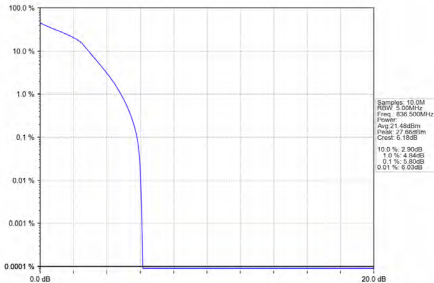
Band26b_3MHz_16QAM_MCH_836.5MHz_RB_15_0_NTNV
