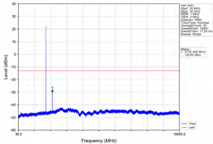
Band4_5MHz_QPSK_MCH_1732.5MHz_RB_1_0_NTNV
