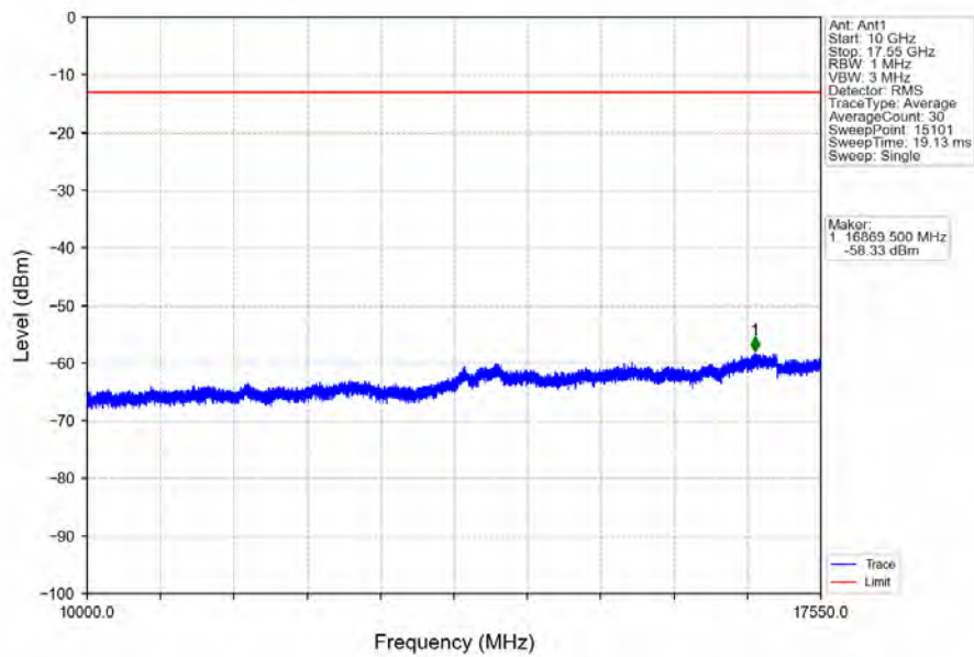
Band4_15MHz_64QAM_LCH_1717.5MHz_RB_75_0_NTNV
