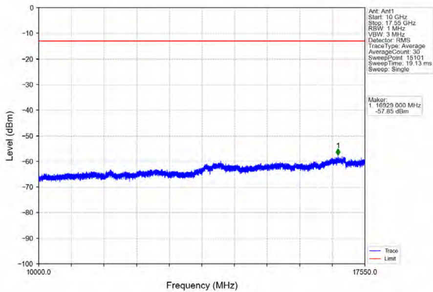
Band4_5MHz_QPSK_LCH_1712.5MHz_RB_25_0_NTNV
