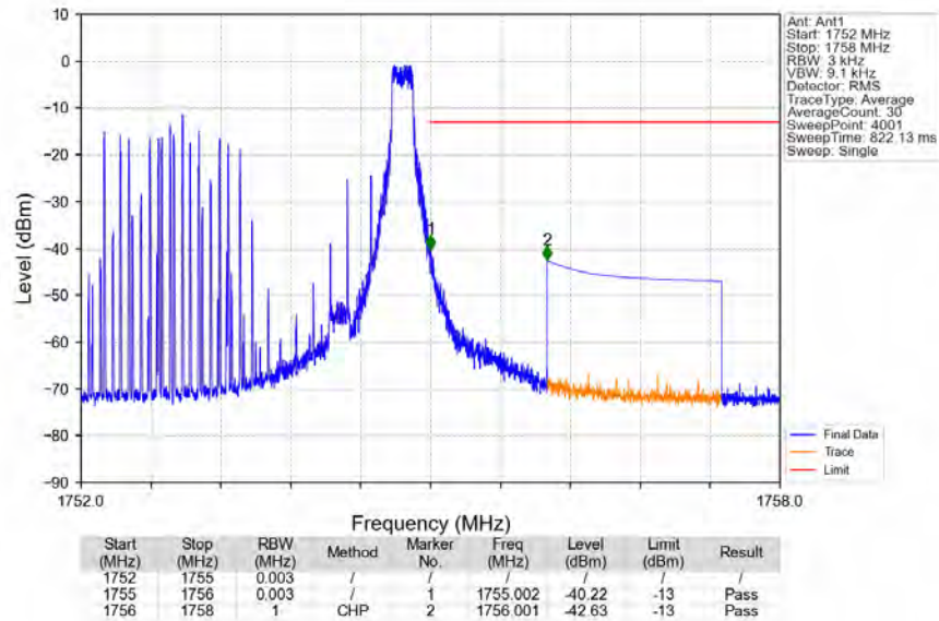
Band4_3MHz_64QAM_HCH_1753.5MHz_RB_1_14_NTNV
