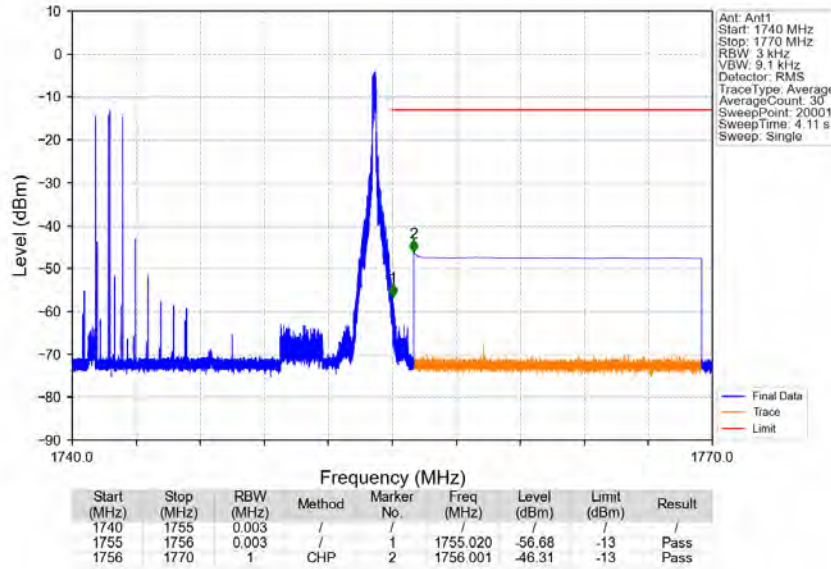
Band4_15MHz_64QAM_HCH_1747.5MHz_RB_1_74_NTNV
