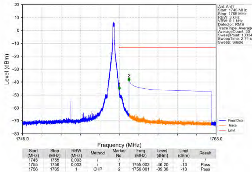
Band4_10MHz_16QAM_HCH_1750MHz_RB_1_49_NTNV
