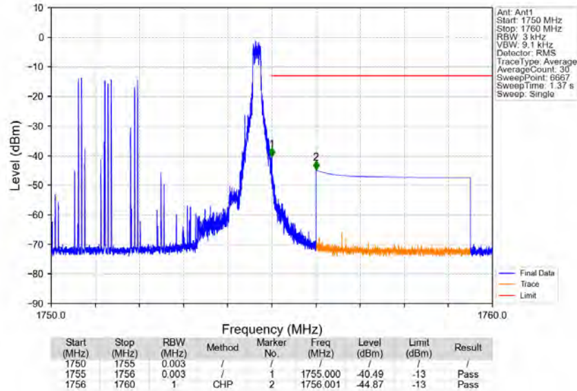
Band4_5MHz_64QAM_HCH_1752.5MHz_RB_1_24_NTNV
