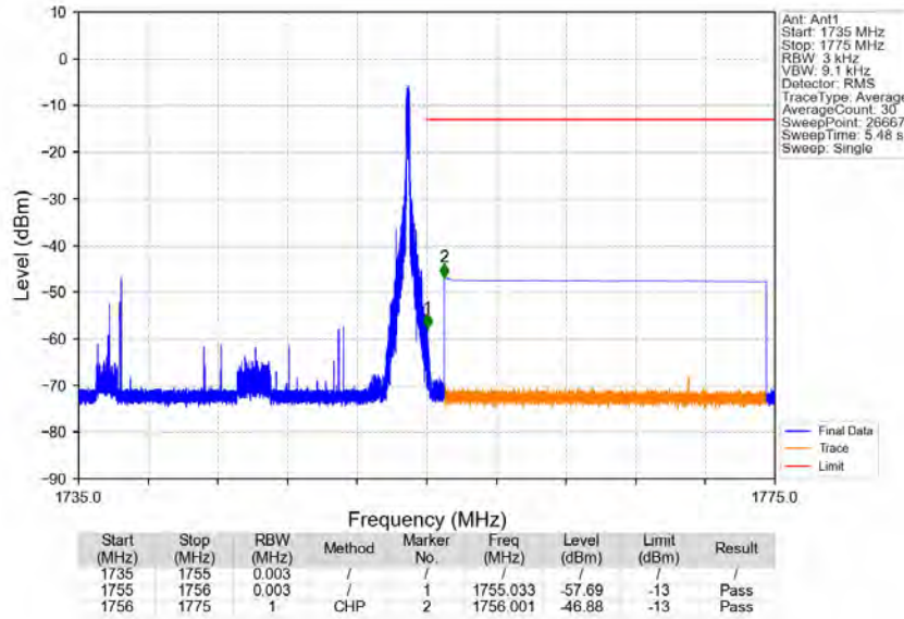
Band4_20MHz_64QAM_HCH_1745MHz_RB_1_99_NTNV
