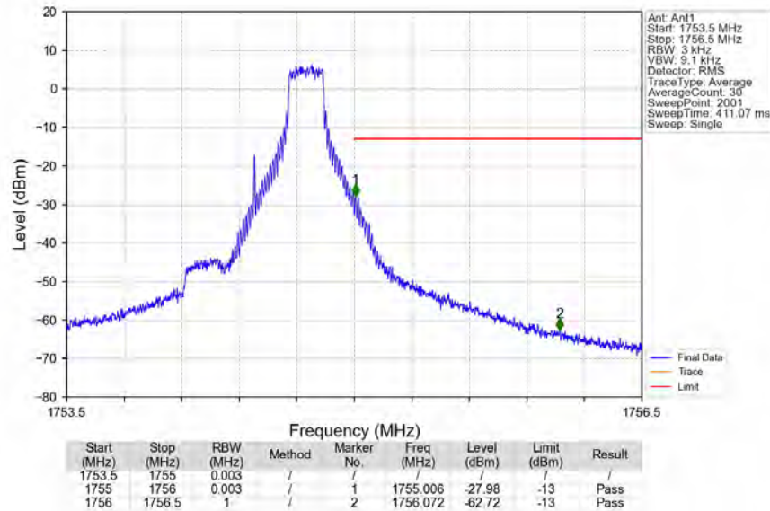
Band4_1.4MHz_16QAM_HCH_1754.3MHz_RB_1_5_NTNV
