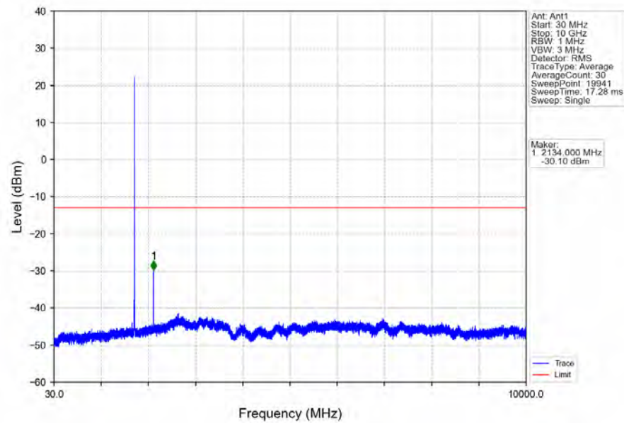
Band4_3MHz_QPSK_MCH_1732.5MHz_RB_1_0_NTNV
