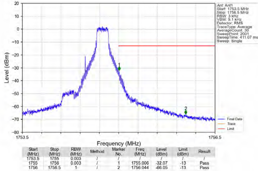
Band4_1.4MHz_64QAM_HCH_1754.3MHz_RB_1_5_NTNV
