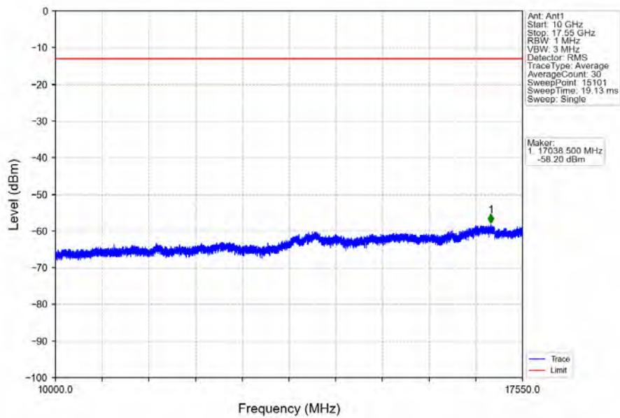
Band4_10MHz_64QAM_LCH_1715MHz_RB_50_0_NTNV
