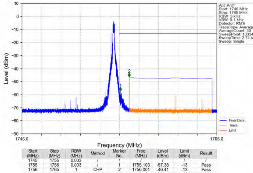
Band4_10MHz_64QAM_HCH_1750MHz_RB_1_49_NTNV
