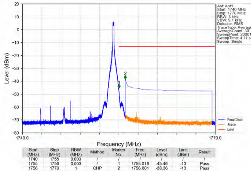
Band4_15MHz_16QAM_HCH_1747.5MHz_RB_1_74_NTNV
