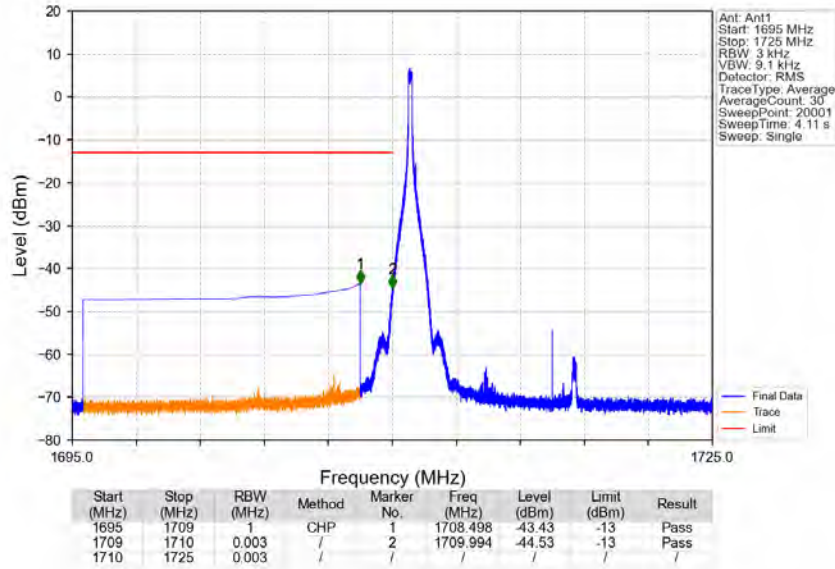
Band4_15MHz_16QAM_LCH_1717.5MHz_RB_1_0_NTNV
