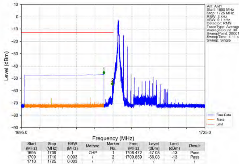
Band4_15MHz_64QAM_LCH_1717.5MHz_RB_1_0_NTNV
