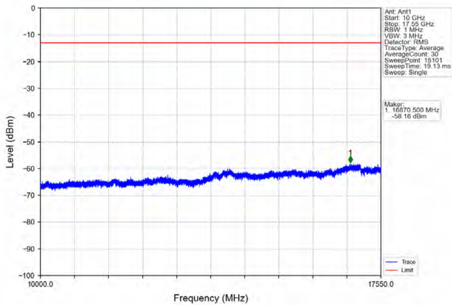
Band4_3MHz_QPSK_LCH_1711.5MHz_RB_15_0_NTNV
