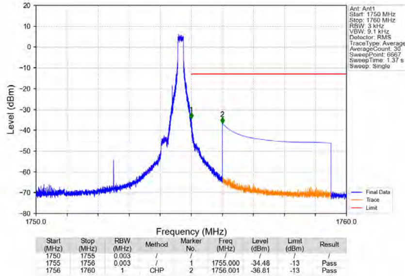
Band4_5MHz_16QAM_HCH_1752.5MHz_RB_1_24_NTNV
