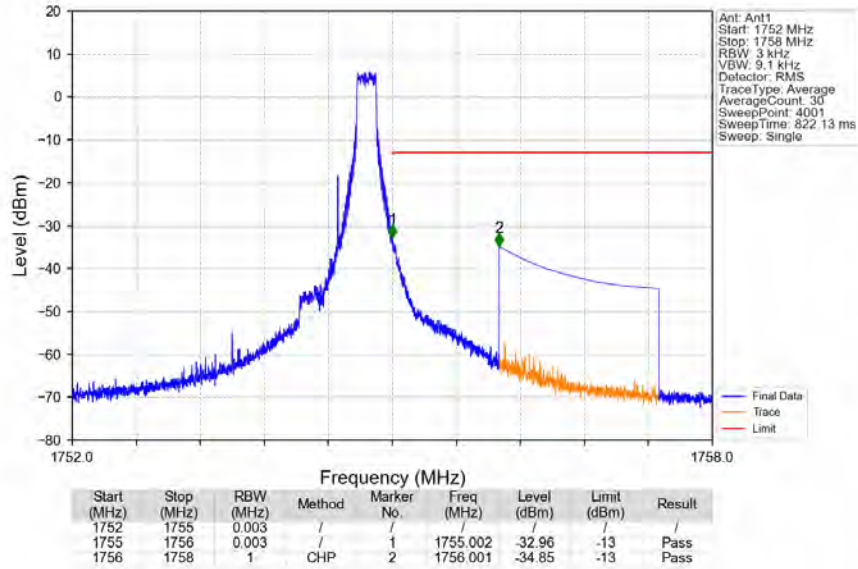
Band4_3MHz_16QAM_HCH_1753.5MHz_RB_1_14_NTNV
