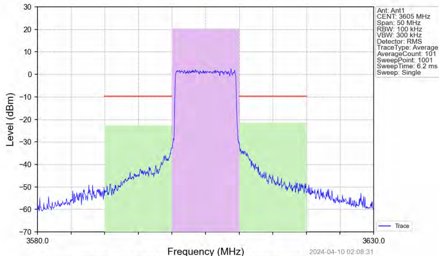
Band43c_10MHz_64QAM_LCH_3605MHz_RB_50_0_NTNV
