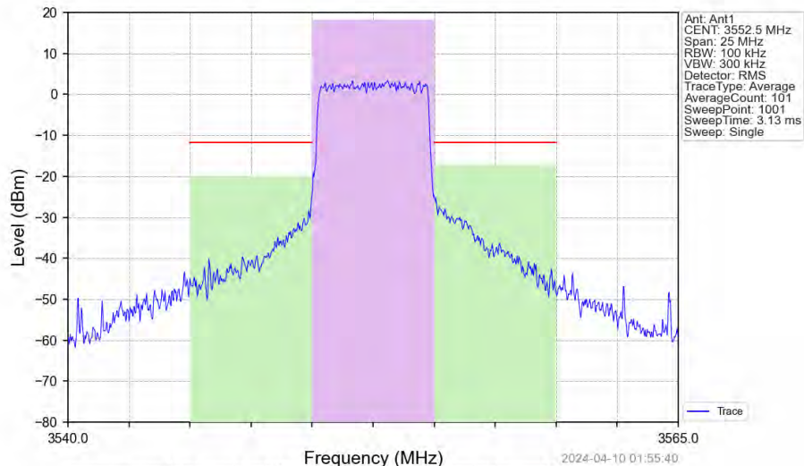
Band42c_5MHz_64QAM_LCH_3552.5MHz_RB_25_0_NTNV
