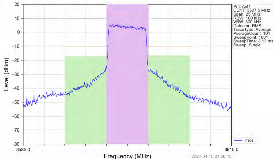
Band42c_5MHz_QPSK_HCH_3597.5MHz_RB_25_0_NTNV
