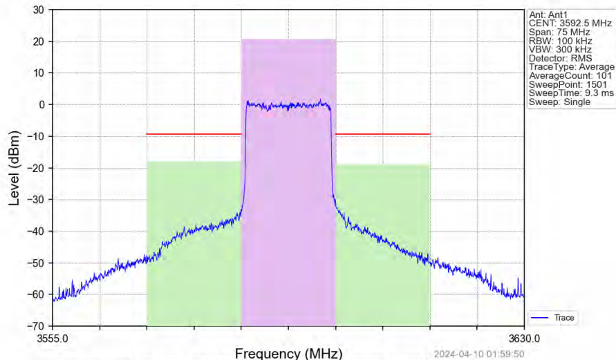
Band42c_15MHz_QPSK_HCH_3592.5MHz_RB_75_0_NTNV
