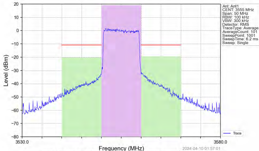
Band42c_10MHz_64QAM_LCH_3555MHz_RB_50_0_NTNV
