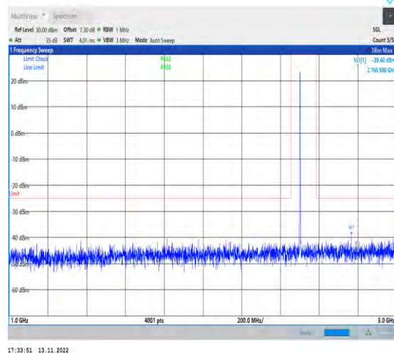
1-N7-PC3-15-40-L-1-DFT-PI2BPSK-Inner_1RB_Left- 1@1-1000-3000-Ant1-2766.50--39.40--25-PASS
