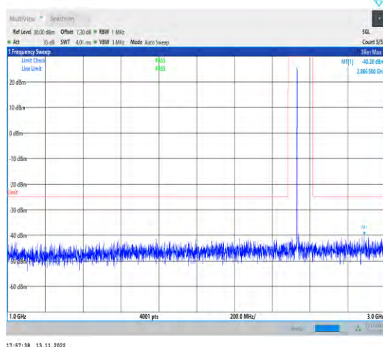
1-N7-PC3-15-40-H-1-DFT-PI2BPSK-Inner_1RB_Left- 1@1-1000-3000-Ant1-2886.50--40.20--25-PASS
