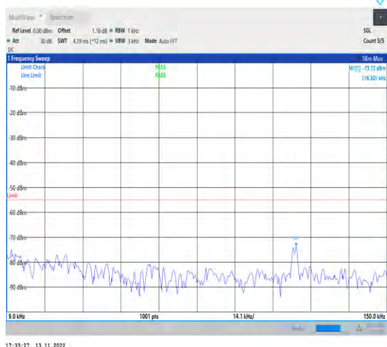
1-N7-PC3-15-40-L-1-DFT-PI2BPSK-Inner_1RB_Left -1@1-0.009-0.15-Ant1-0.12--73.72--55-PASS
