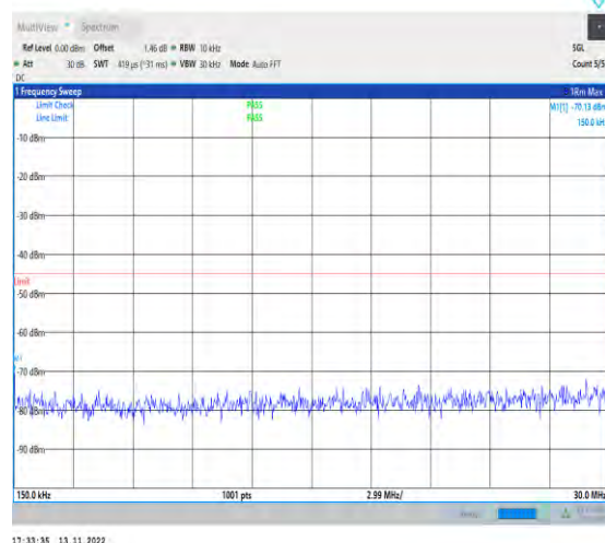
1-N7-PC3-15-40-L-1-DFT-PI2BPSK-Inner_1RB_Left- 1@1-0.15-30-Ant1-0.15--70.13--45-PASS
