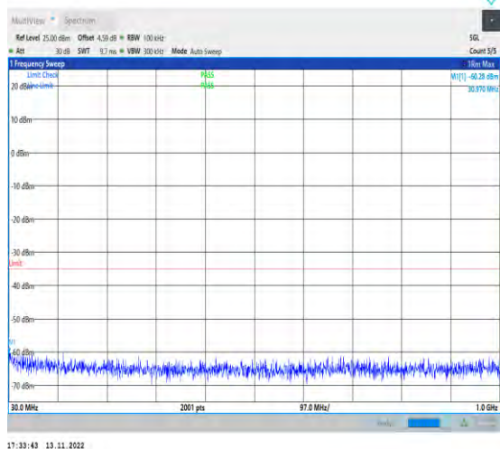
1-N7-PC3-15-40-L-1-DFT-PI2BPSK-Inner_1RB_Left -1@1-30-1000-Ant1-30.97--60.28--35-PASS
