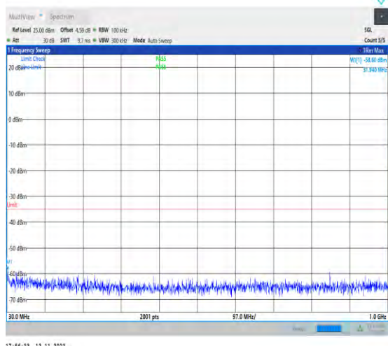
1-N7-PC3-15-40-M-1-DFT-PI2BPSK-Inner_1RB_Lef t-1@1-30-1000-Ant1-31.94--58.80--35-PASS
