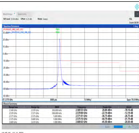
1-N7-PC3-15-30-H-2-DFT-PI2BPSK-Edge_1RB_Right-1@159-Ant1-1--PASS-see graph
