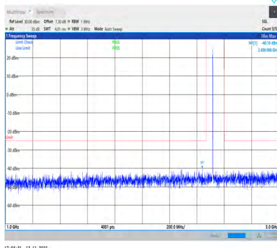
1-N7-PC3-15-40-M-1-DFT-PI2BPSK-Inner_1RB_Left- 1@1-1000-3000-Ant1-2439.00--40.19--25-PASS
