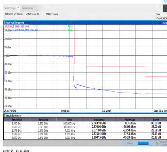
1-N7-PC3-15-30-H-6-CP-QPSK-Outer_Full-160@0-Ant1-1--PASS-see graph
