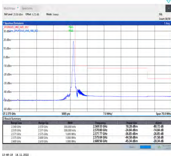
1-N7-PC3-15-30-H-5-CP-QPSK-Edge_1RB_Right-1@159-Ant1-1--PASS-see graph
