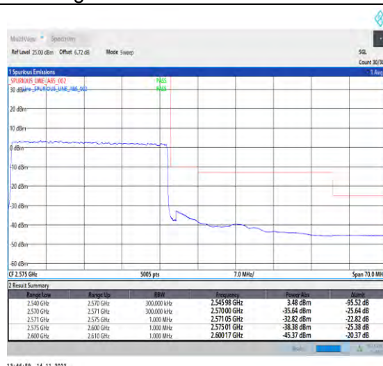
1-N7-PC3-15-30-H-3-DFT-PI2BPSK-Outer_Full-160@0-Ant1-1--PASS-see graph
