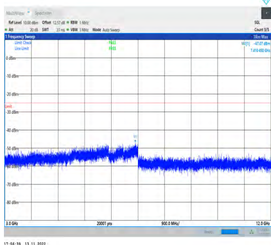
1-N7-PC3-15-40-M-1-DFT-PI2BPSK-Inner_1RB_Lef t-1@1-3000-12000-Ant1-7410.45--47.07--25-PASS
