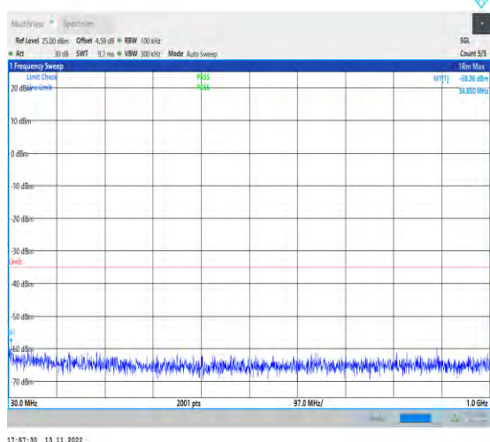
1-N7-PC3-15-40-H-1-DFT-PI2BPSK-Inner_1RB_Lef t-1@1-30-1000-Ant1-34.85--58.36--35-PASS
