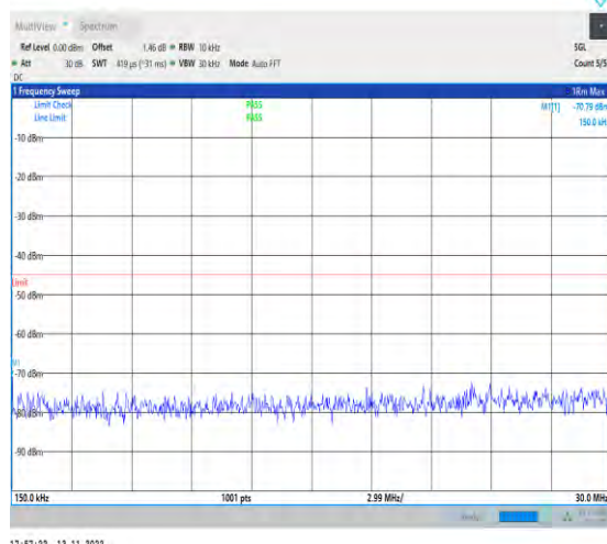
1-N7-PC3-15-40-H-1-DFT-PI2BPSK-Inner_1RB_Left- 1@1-0.15-30-Ant1-0.15--70.79--45-PASS
