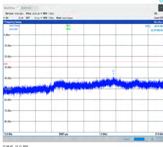
1-N7-PC3-15-40-M-1-DFT-PI2BPSK-Inner_1RB_Left- 1@1-12000-27000-Ant1-22275.00--36.74--25-PASS
