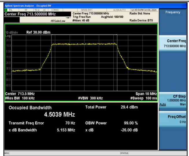
Band12-5MHz-256QAM-23155-25RB#0-PASS
