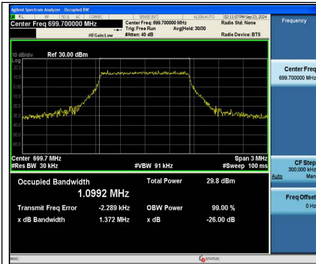
Band12-1.4MHz-64QAM-23017-6RB#0-PASS
