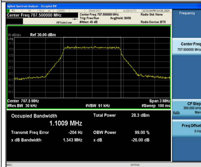
Band12-1.4MHz-256QAM-23095-6RB#0-PASS
