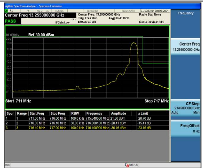
Band12-5MHz-QPSK-23155-1RB#24-PASS
