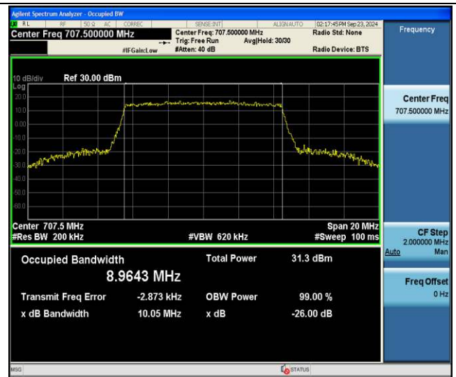
Band12-10MHz-64QAM-23095-50RB#0-PASS
