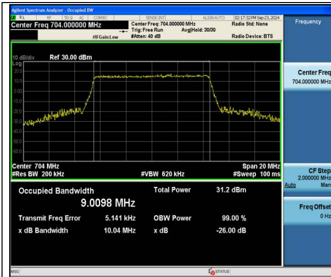
Band12-10MHz-64QAM-23060-50RB#0-PASS
