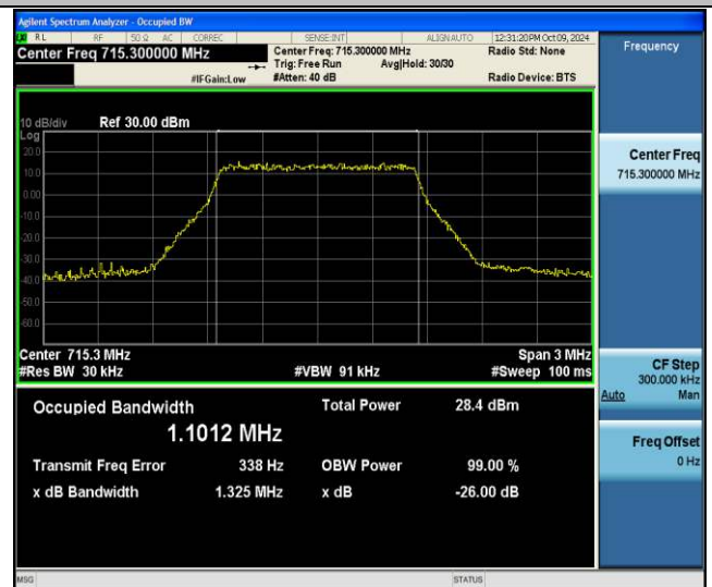
Band12-1.4MHz-256QAM-23173-6RB#0-PASS
