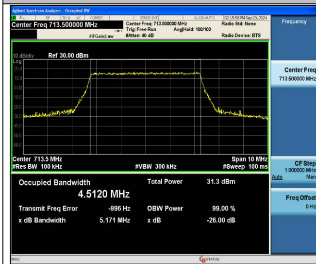
Band12-5MHz-64QAM-23155-25RB#0-PASS
