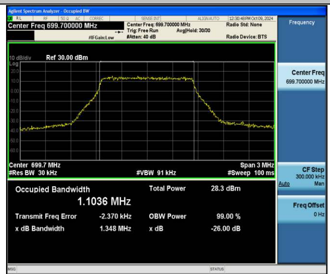
Band12-1.4MHz-256QAM-23017-6RB#0-PASS
