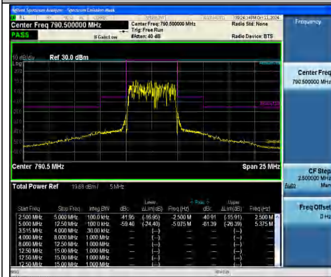
NTNV-Band14-5MHz-256QAM-23305-25RB#0--12.50--5.00-PASS
