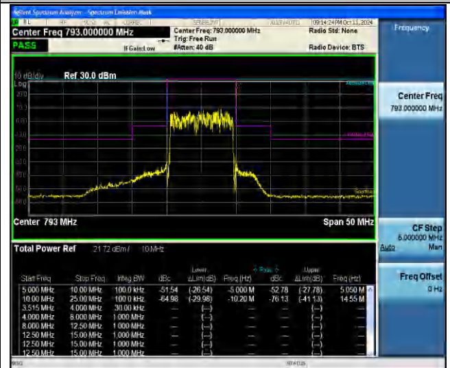
NTNV-Band14-10MHz-64QAM-23330-50RB#0--25.00--10.00-PASS
