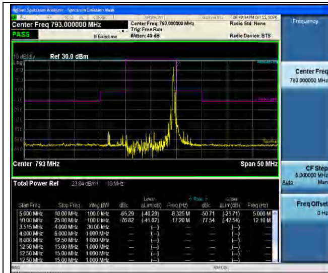
NTNV-Band14-10MHz-16QAM-23330-1RB#49-10.00-25.00-PASS
