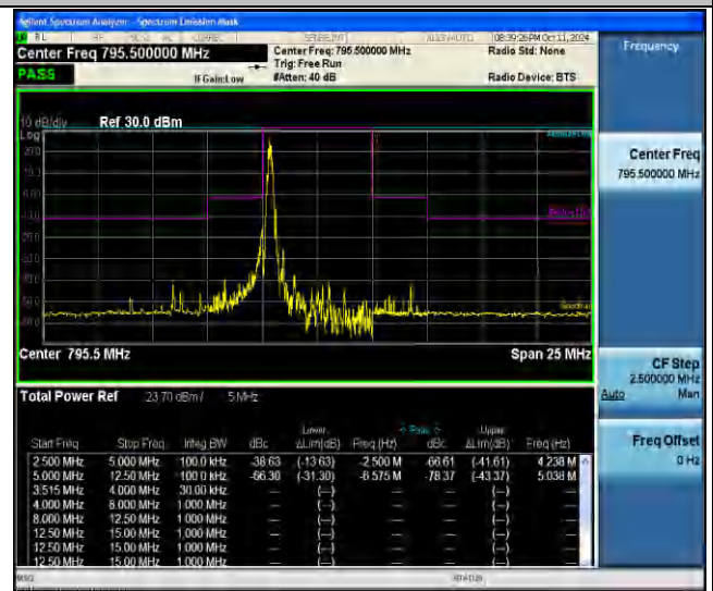
NTNV-Band14-5MHz-16QAM-23355-1RB#0-2.50-5.00-PASS
