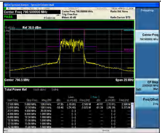
NTNV-Band14-5MHz-256QAM-23305-25RB#0--5.00--2.50-PASS
