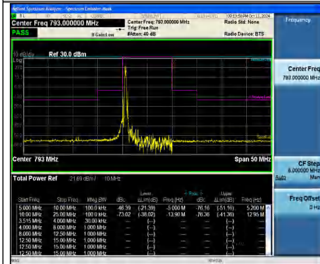
NTNV-Band14-10MHz-64QAM-23330-1RB#0-10.00-25.00-PASS
