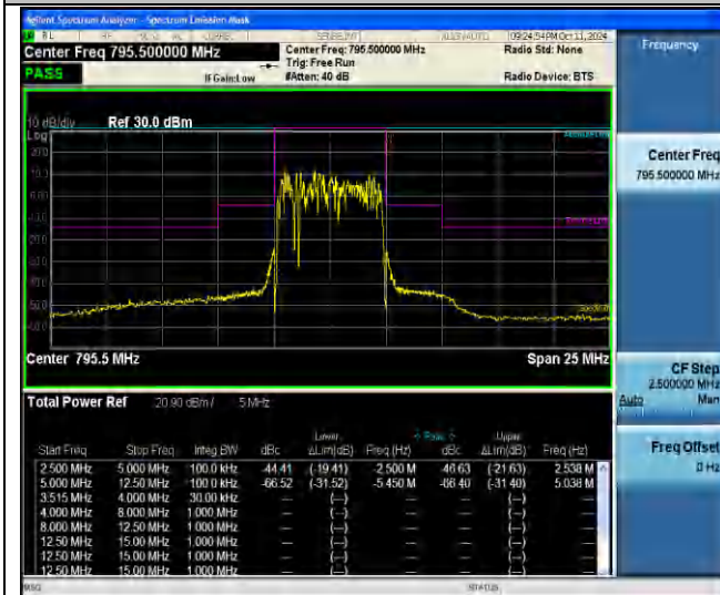
NTNV-Band14-5MHz-256QAM-23355-25RB#0--12.50--5.00-PASS
