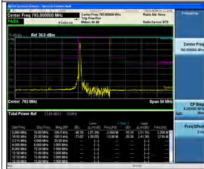
NTNV-Band14-10MHz-64QAM-23330-1RB#0--10.00--5.00-PASS
