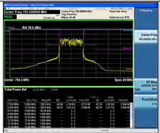
NTNV-Band14-5MHz-16QAM-23355-25RB#0--12.50--5.00-PASS
