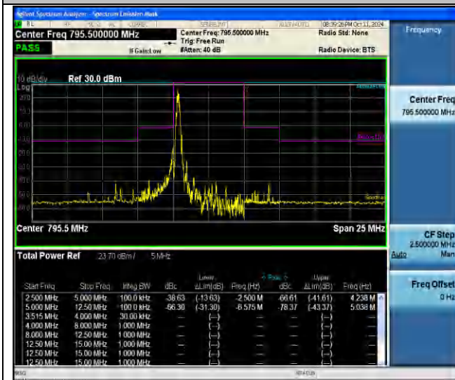
NTNV-Band14-5MHz-16QAM-23355-1RB#0-5.00-12.50-PASS
