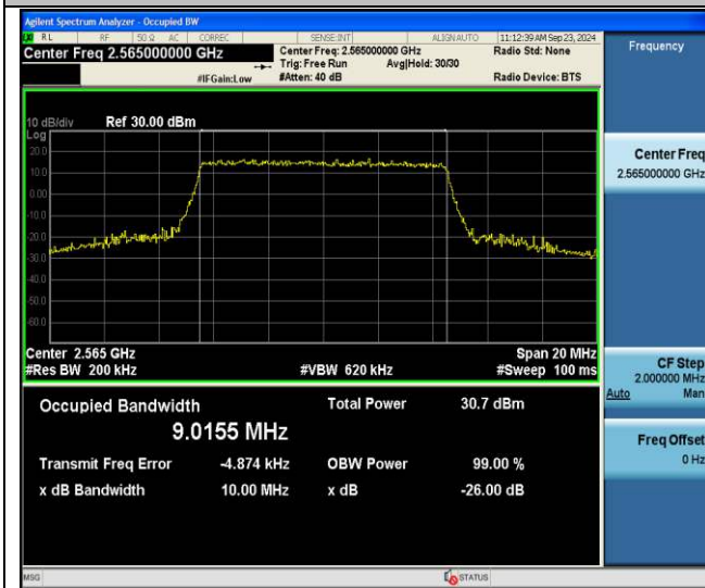
Band7-10MHz-64QAM-21400-50RB#0-PASS
