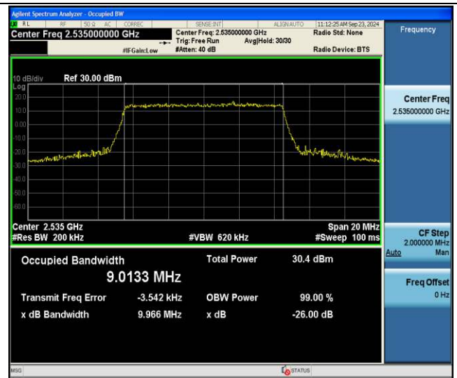
Band7-10MHz-64QAM-21100-50RB#0-PASS
