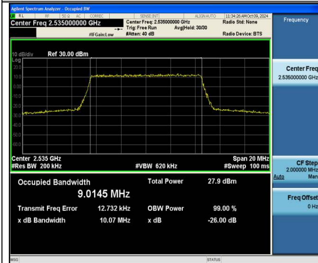
Band7-10MHz-256QAM-21100-50RB#0-PASS
