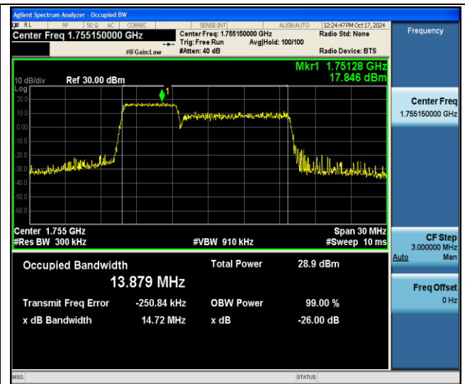
66-66-5MHz-10MHz-64QAM-64QAM-132375-132447-25RB#0-50RB#0-PASS
