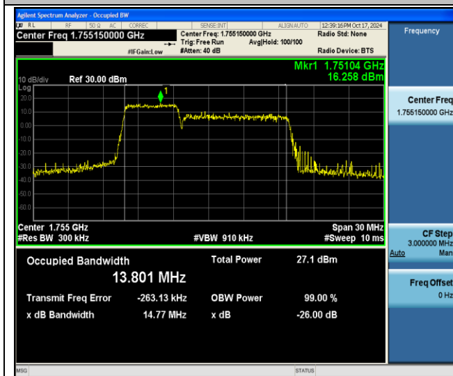
66-66-5MHz-10MHz-256QAM-256QAM-132375-132447-25RB#0-50RB#0-PASS
