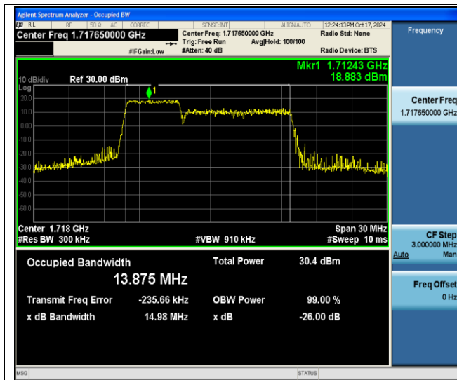
66-66-5MHz-10MHz-64QAM-64QAM-132000-132072-25RB#0-50RB#0-PASS
