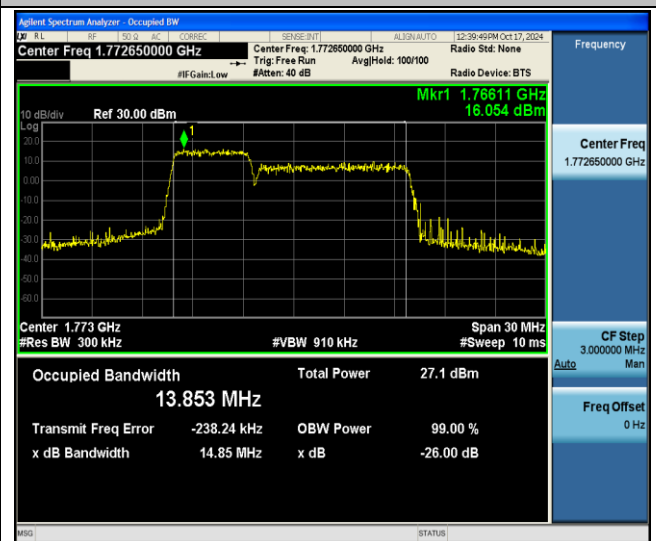
66-66-5MHz-10MHz-256QAM-256QAM-132550-132622-25RB#0-50RB#0-PASS
