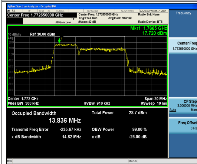
66-66-5MHz-10MHz-64QAM-64QAM-132550-132622-25RB#0-50RB#0-PASS
