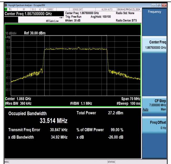
NTNV-n2-PC3-15-35-L-CP-256QAM-Outer_Full-Ant1-PASS
