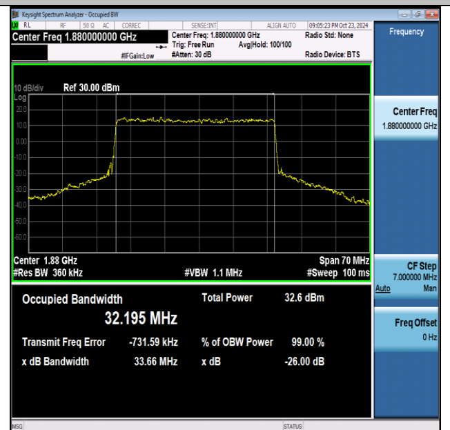
NTNV-n2-PC3-15-35-M-DFT-QPSK-Outer_Full-Ant1-PASS
