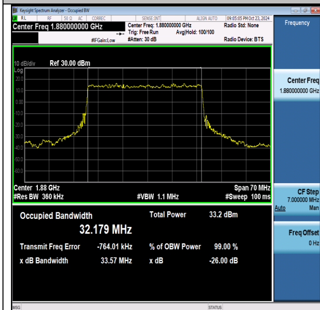
NTNV-n2-PC3-15-35-M-DFT-BPSK-Outer_Full-Ant1-PASS
