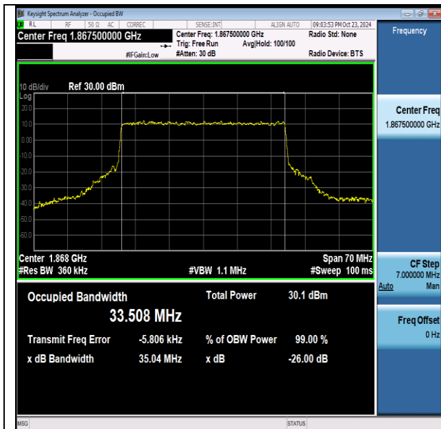
NTNV-n2-PC3-15-35-L-CP-64QAM-Outer_Full-Ant1-PASS
