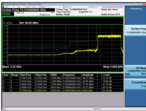
NTNV-n38-PC3-30-15-L-DFT-BPSK-Outet_Full-PASS
