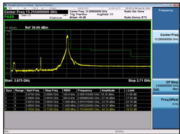
NTNV-n41-PC2-30-15-H-CP-QPSK-Edge_1RB_Right-PASS
