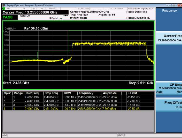
NTNV-n41-PC2-30-15-L-DFT-BPSK-Outer_Full-PASS
