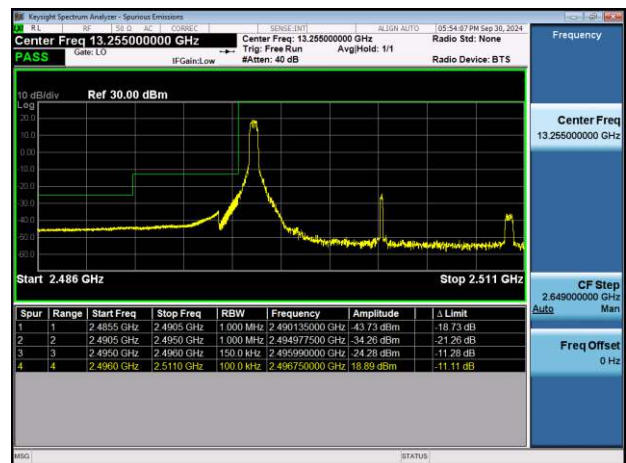
NTNV-n41-PC2-30-15-L-CP-QPSK-Edge_1RB_Left-PASS
