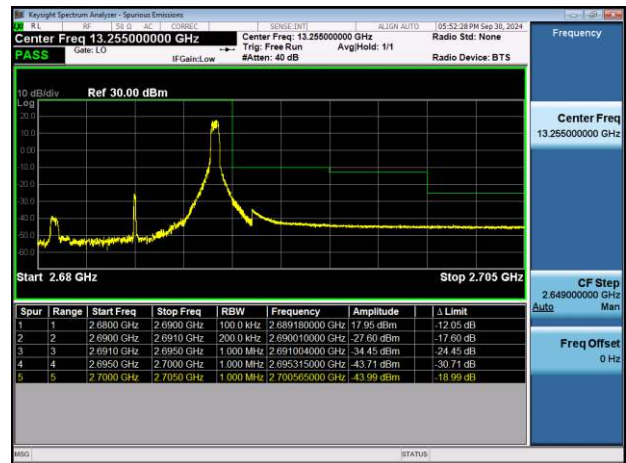
NTNV-n41-PC2-30-10-H-CP-QPSK-Edge_1RB_Right-PASS
