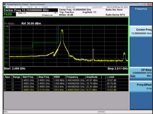
NTNV-n41-PC2-30-15-L-DFT-BPSK-Edge_1RB_Left-PASS
