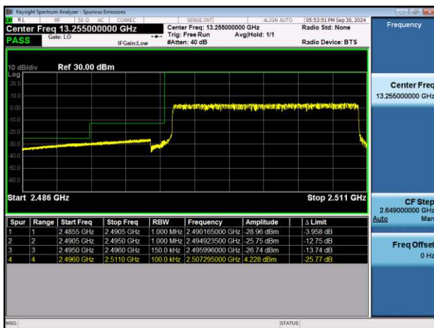
NTNV-n41-PC2-30-15-L-CP-QPSK-Outer_Full-PASS
