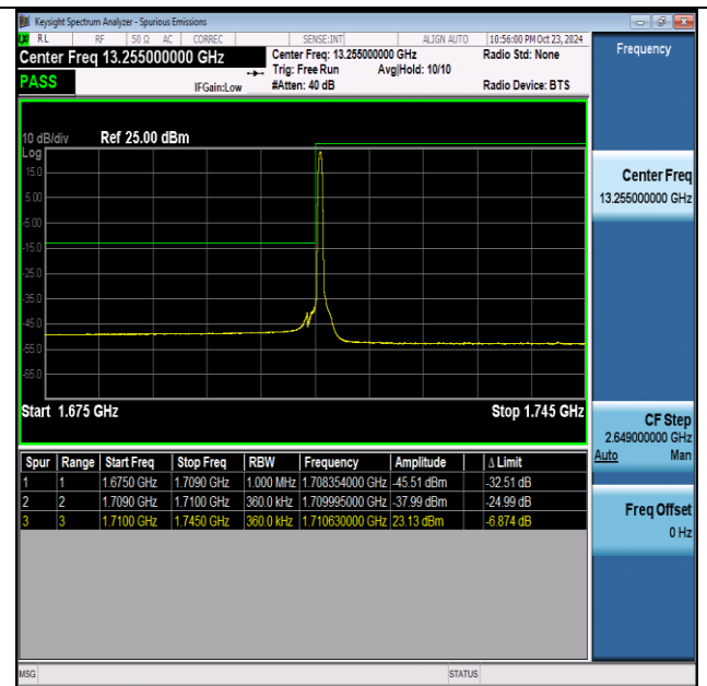
NTNV-n66-PC3-15-35-L-DFT-BPSK-Edge_1RB_Left-PASS
