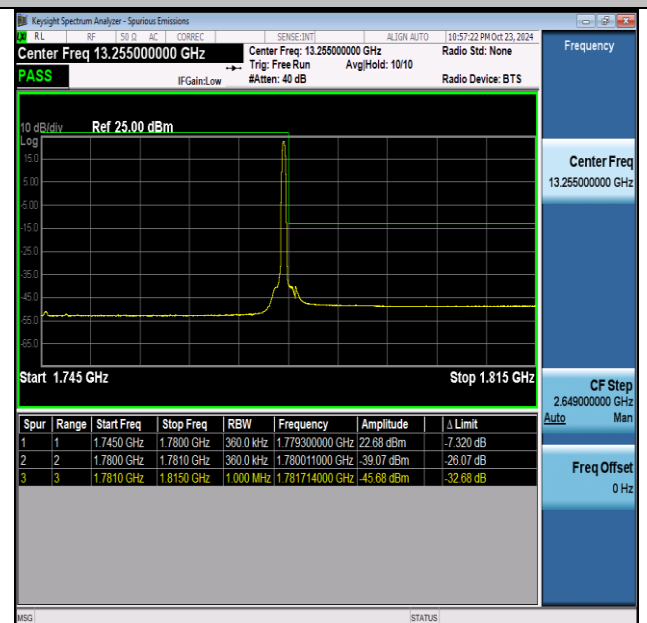
NTNV-n66-PC3-15-35-H-DFT-BPSK-Edge_1RB_Right-PASS
