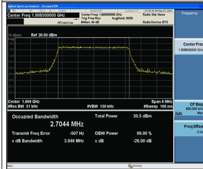
Band2-3MHz-64QAM-19185-15RB#0-PASS
