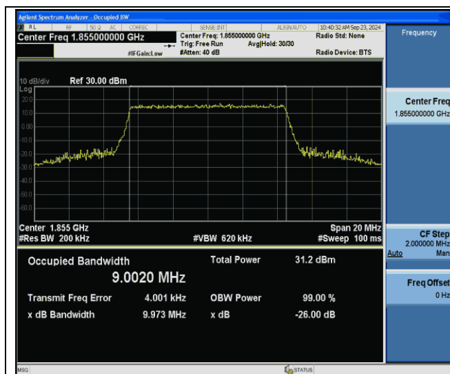
Band2-10MHz-64QAM-18650-50RB#0-PASS
