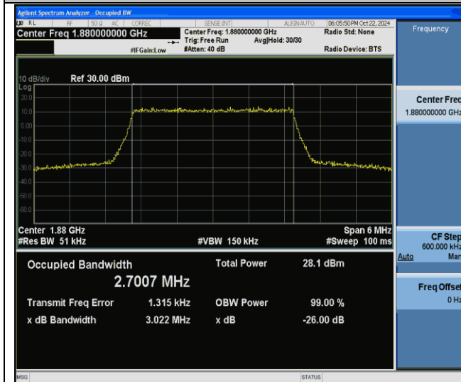
Band2-3MHz-256QAM-18900-15RB#0-PASS
