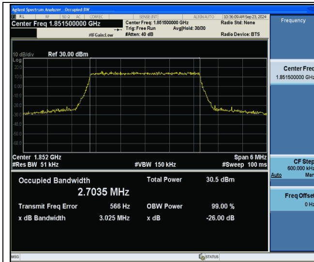
Band2-3MHz-64QAM-18615-15RB#0-PASS
