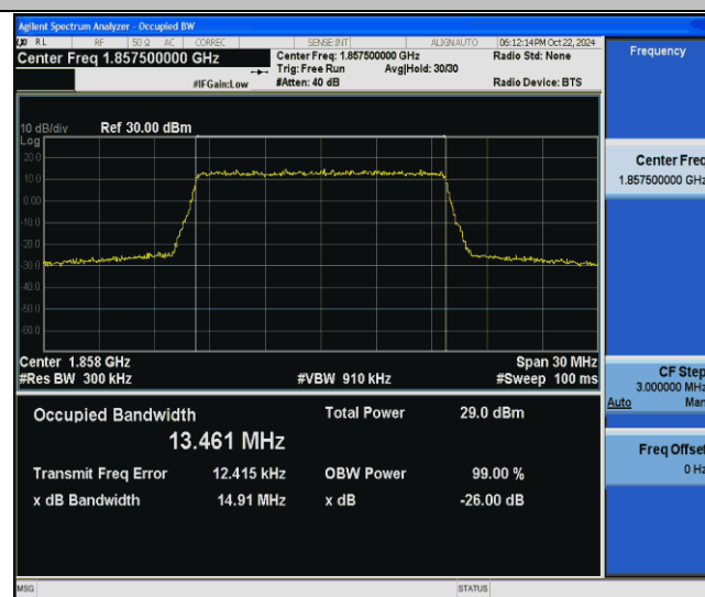
Band2-15MHz-256QAM-18675-75RB#0-PASS
