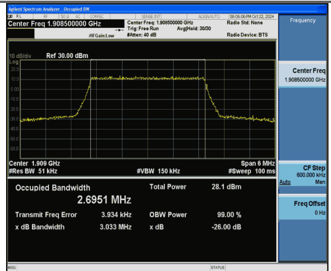
Band2-3MHz-256QAM-19185-15RB#0-PASS
