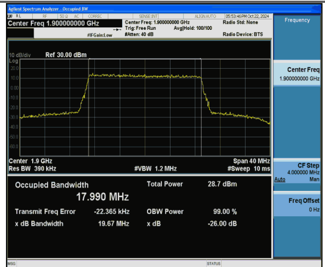
Band2-20MHz-256QAM-19100-100RB#0-PASS
