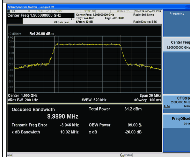
Band2-10MHz-64QAM-19150-50RB#0-PASS
