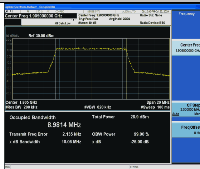
Band2-10MHz-256QAM-19150-50RB#0-PASS
