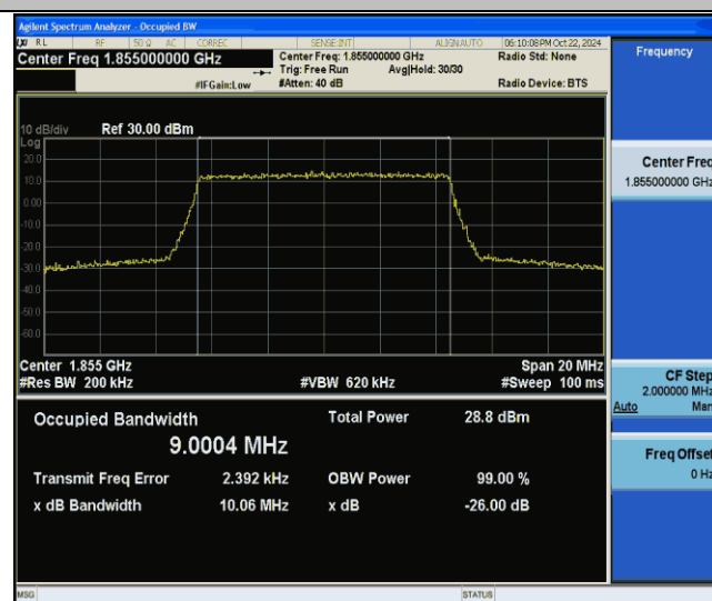
Band2-10MHz-256QAM-18650-50RB#0-PASS
