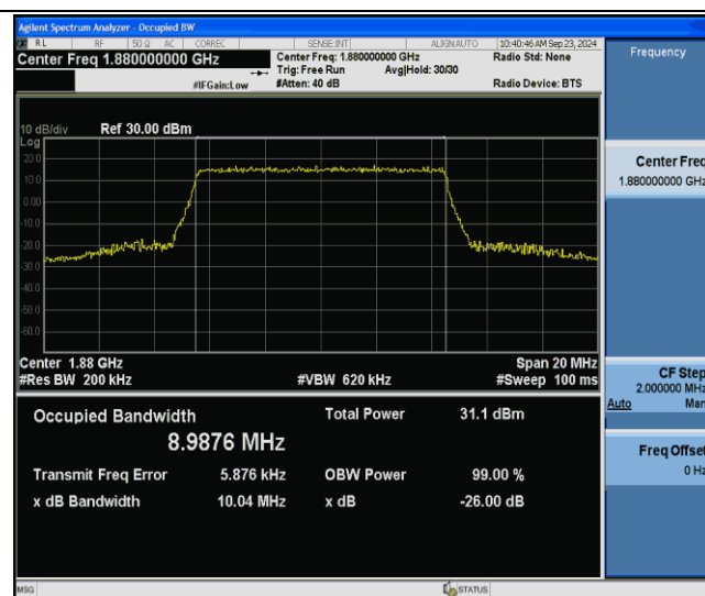
Band2-10MHz-64QAM-18900-50RB#0-PASS
