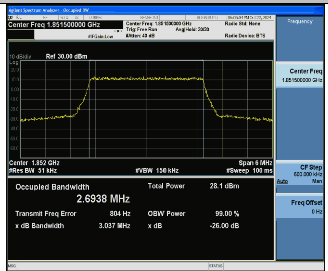
Band2-3MHz-256QAM-18615-15RB#0-PASS
