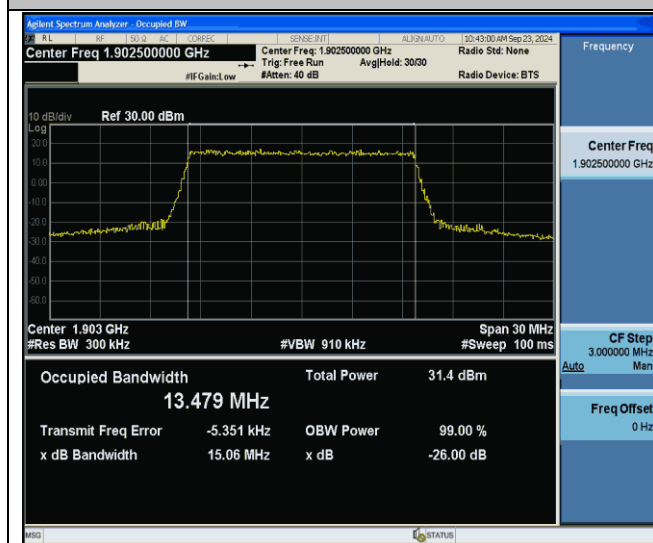
Band2-15MHz-64QAM-19125-75RB#0-PASS
