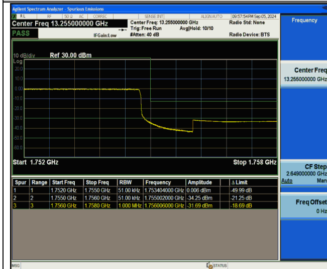
Band4-5MHz-QPSK-20375-25RB#0-PASS
