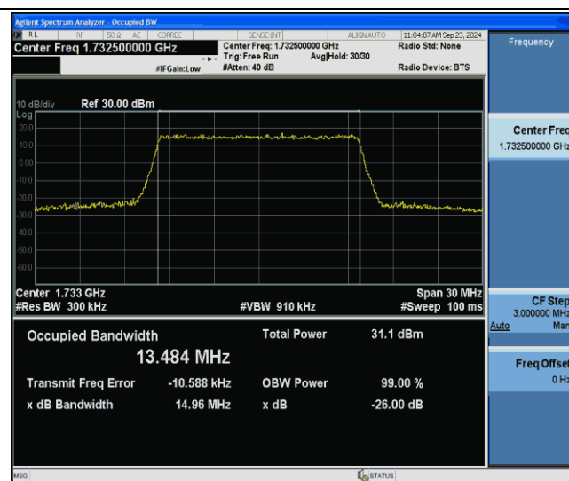
Band4-15MHz-64QAM-20175-75RB#0-PASS
