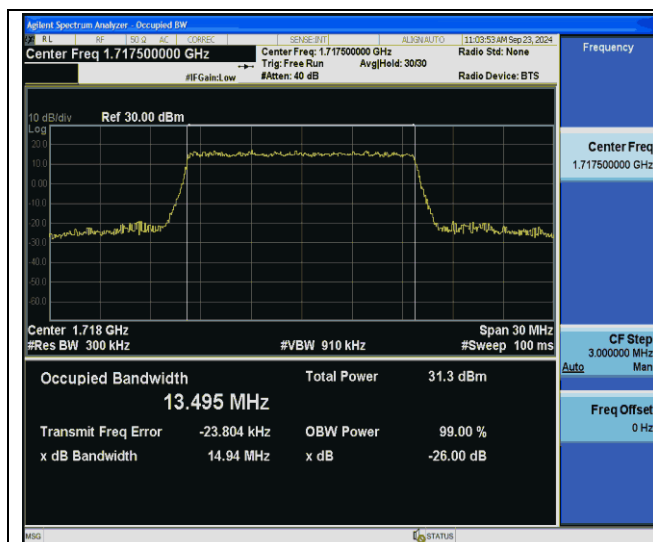
Band4-15MHz-64QAM-20025-75RB#0-PASS
