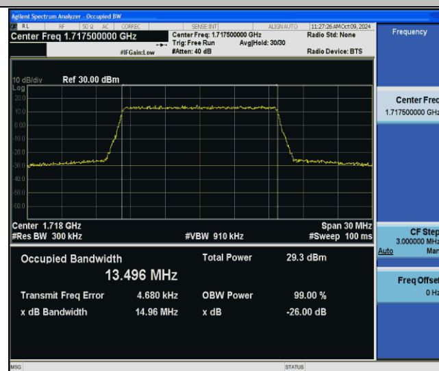
Band4-15MHz-256QAM-20025-75RB#0-PASS
