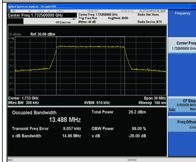
Band4-15MHz-256QAM-20175-75RB#0-PASS
