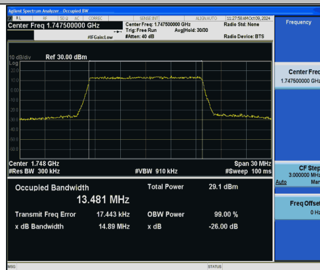
Band4-15MHz-256QAM-20325-75RB#0-PASS
