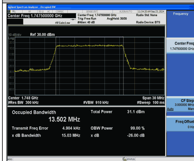
Band4-15MHz-64QAM-20325-75RB#0-PASS
