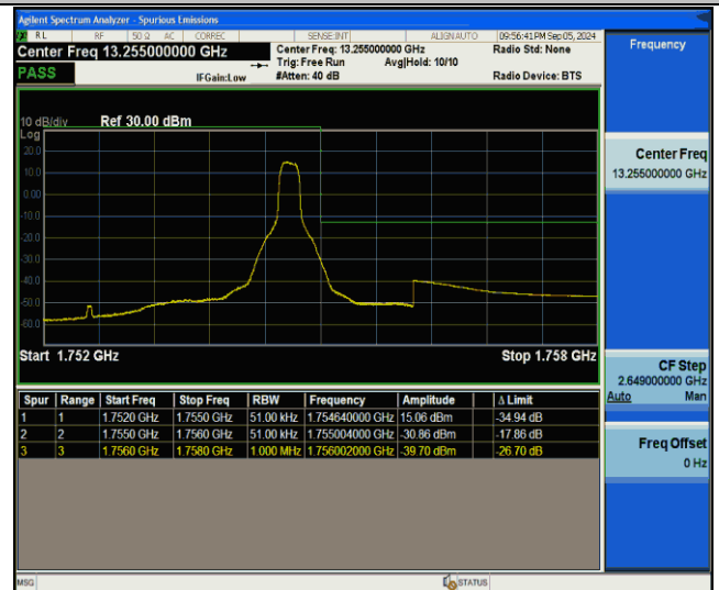
Band4-5MHz-QPSK-20375-1RB#24-PASS
