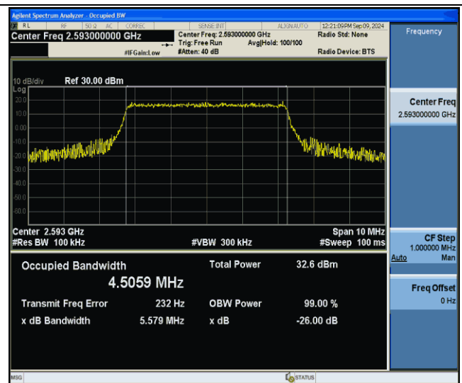
Band41-5MHz-64QAM-40620-25RB#0-PASS
