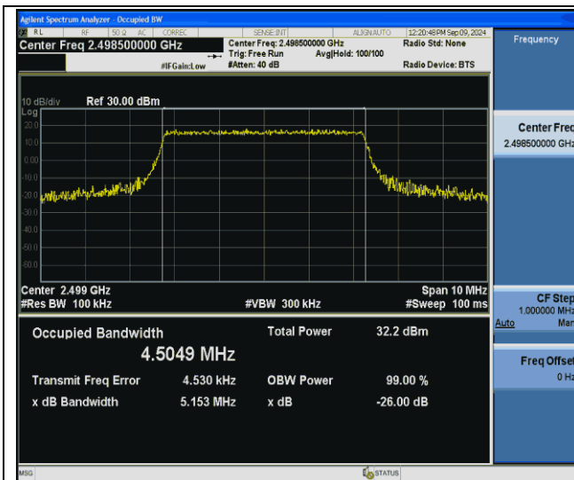
Band41-5MHz-64QAM-39675-25RB#0-PASS
