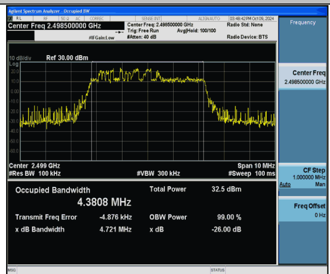
Band41-5MHz-256QAM-39675-25RB#0-PASS
