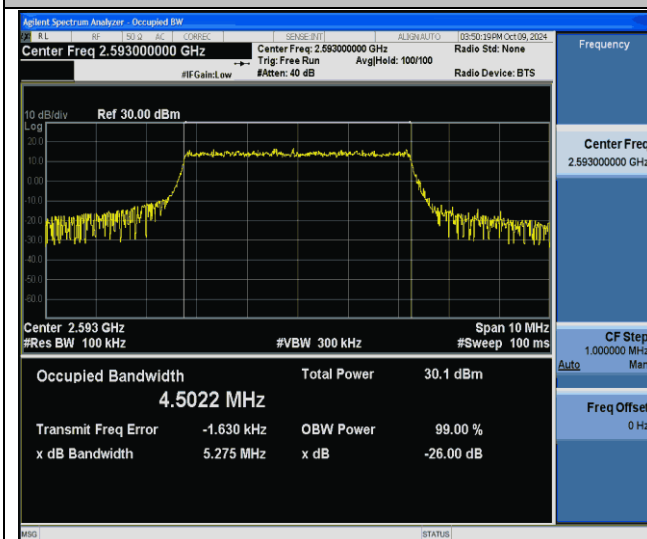
Band41-5MHz-256QAM-40620-25RB#0-PASS
