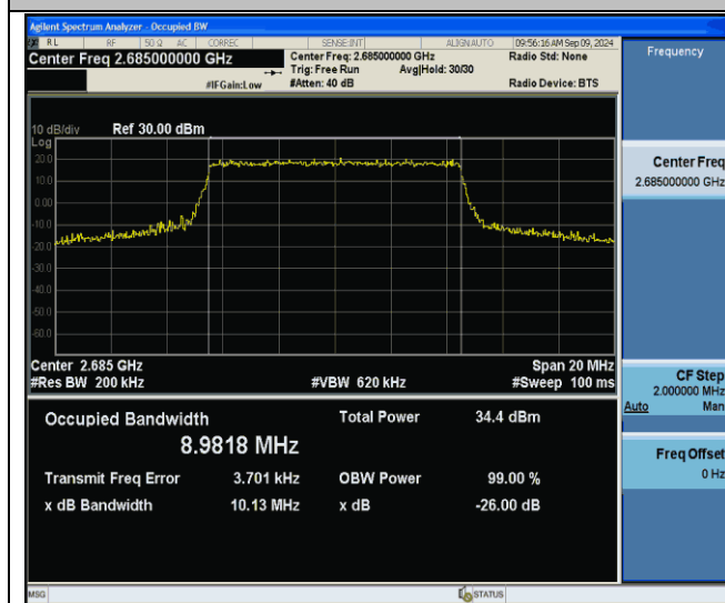
Band41-10MHz-QPSK-41540-50RB#0-PASS
