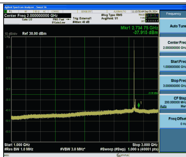
Band41-20MHz-QPSK-41490-1RB#0-1000~3000-PASS
