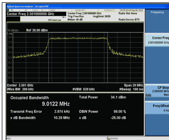
Band41-10MHz-QPSK-39700-50RB#0-PASS
