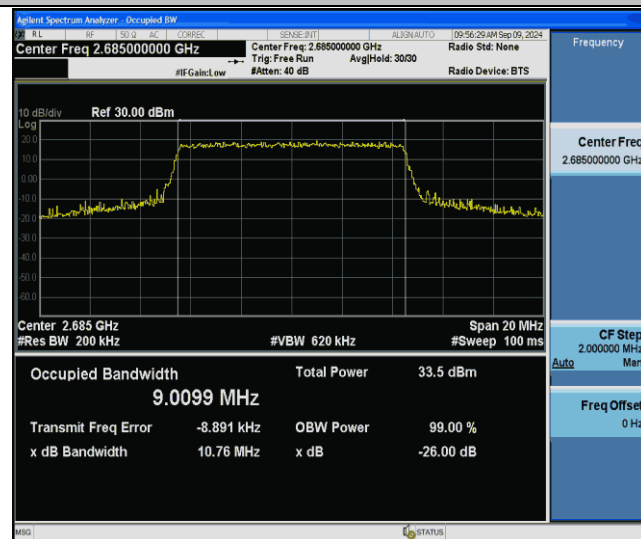
Band41-10MHz-16QAM-41540-50RB#0-PASS
