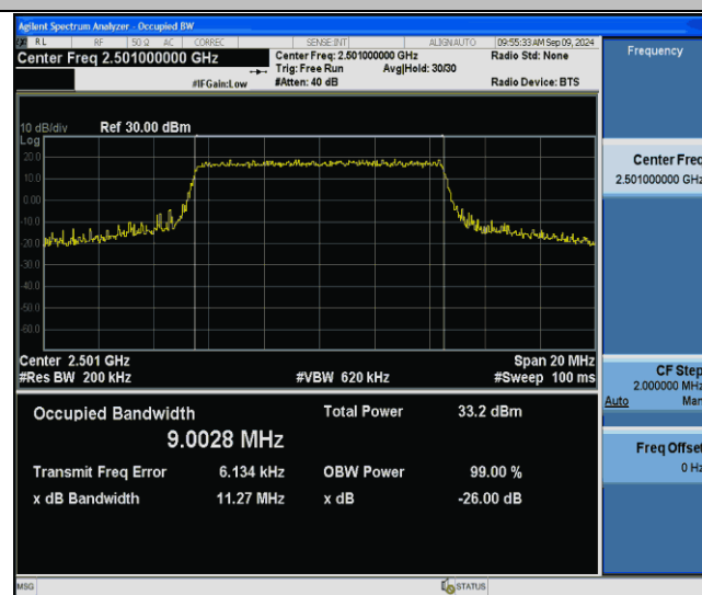
Band41-10MHz-16QAM-39700-50RB#0-PASS
