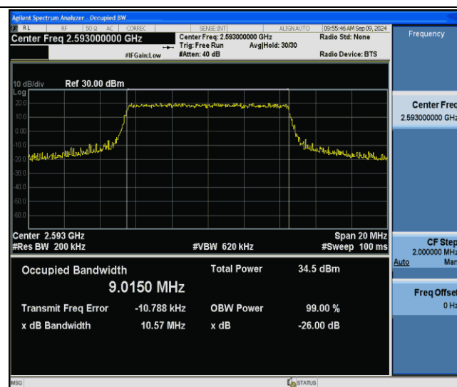
Band41-10MHz-QPSK-40620-50RB#0-PASS
