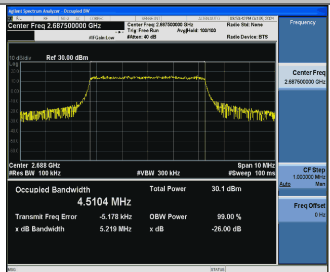
Band41-5MHz-256QAM-41565-25RB#0-PASS
