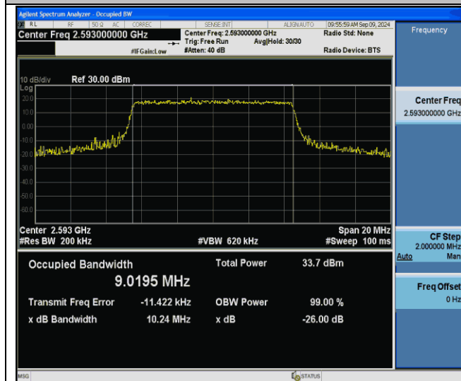
Band41-10MHz-16QAM-40620-50RB#0-PASS
