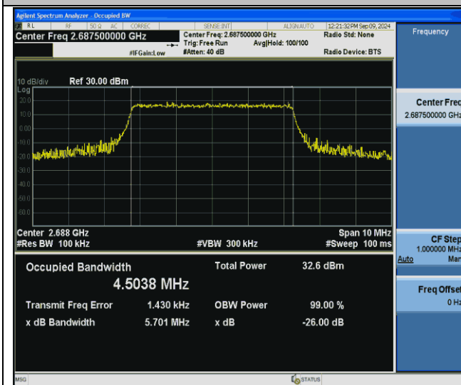
Band41-5MHz-64QAM-41565-25RB#0-PASS
