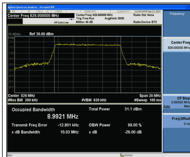
Band5-10MHz-64QAM-20450-50RB#0-PASS
