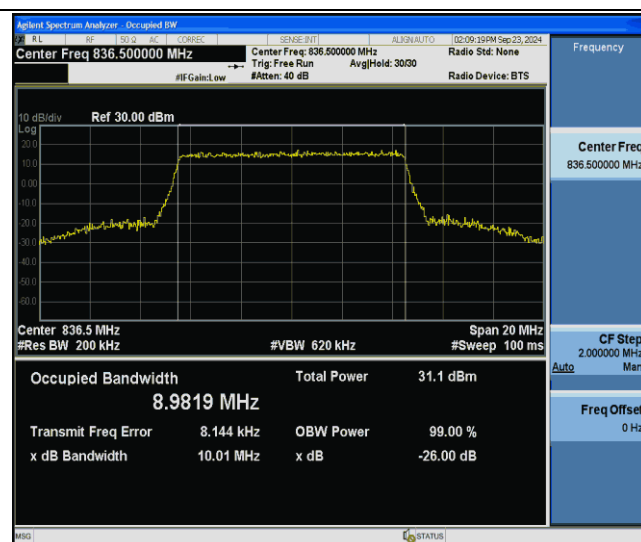
Band5-10MHz-64QAM-20525-50RB#0-PASS
