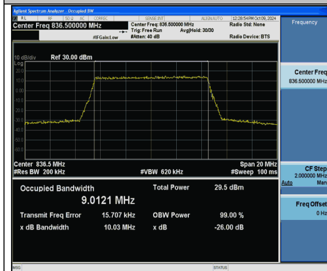
Band5-10MHz-256QAM-20525-50RB#0-PASS
