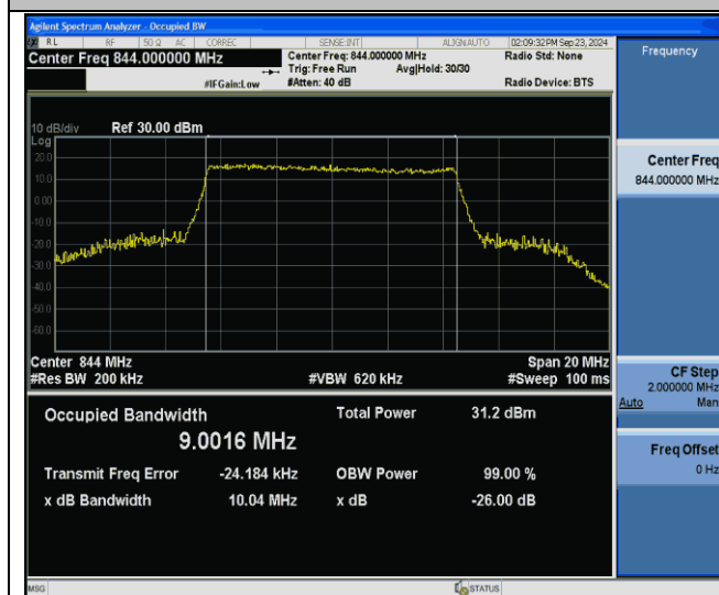
Band5-10MHz-64QAM-20600-50RB#0-PASS
