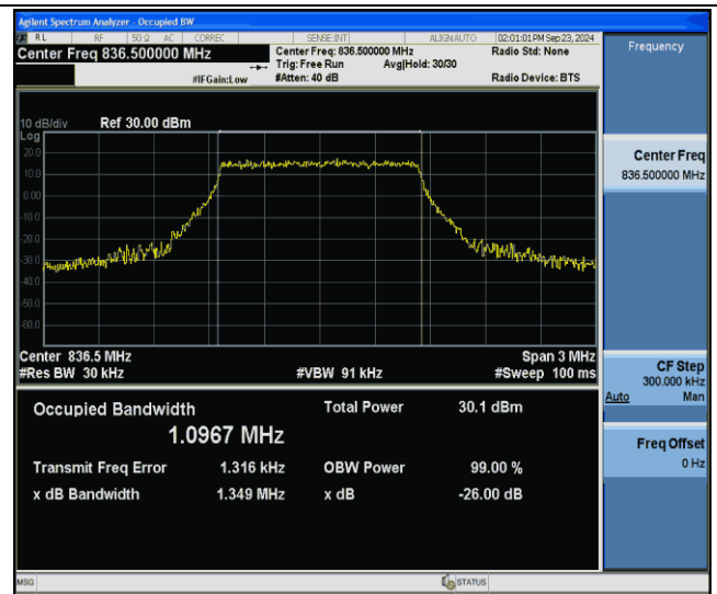
Band5-1.4MHz-64QAM-20525-6RB#0-PASS
