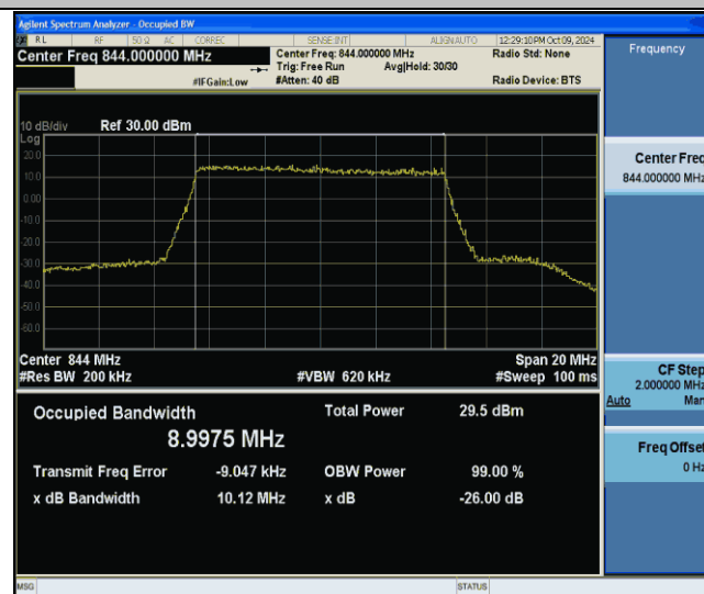
Band5-10MHz-256QAM-20600-50RB#0-PASS
