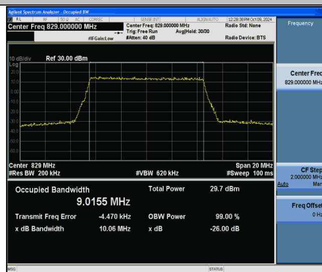
Band5-10MHz-256QAM-20450-50RB#0-PASS
