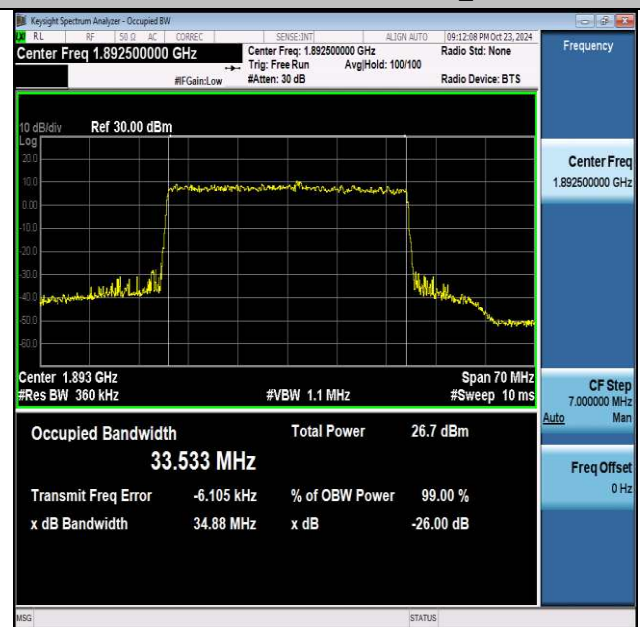
NTNV-n2-PC3-15-35-H-CP-256QAM-Outer_Full-Ant1-PASS
