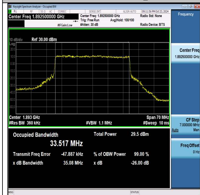
NTNV-n2-PC3-15-35-H-CP-64QAM-Outer_Full-Ant1-PASS
