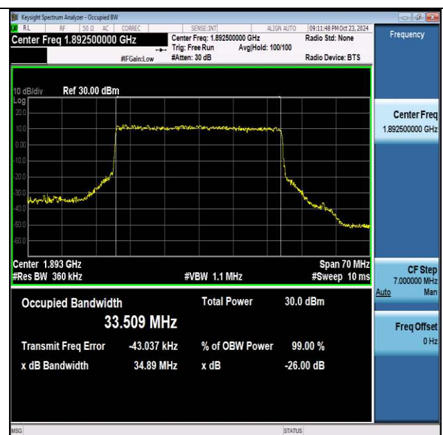
NTNV-n2-PC3-15-35-H-CP-16QAM-Outer_Full-Ant1-PASS
