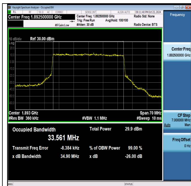
NTNV-n2-PC3-15-35-H-CP-QPSK-Outer_Full-Ant1-PASS
