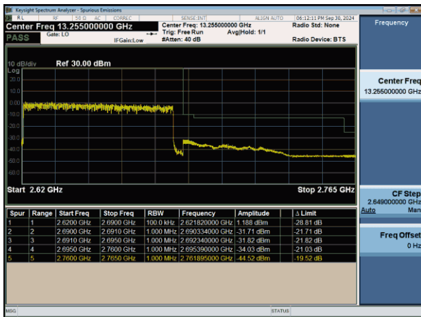
NTNV-n41-PC2-30-70-H-DFT-BPSK-Outer_Full-PASS
