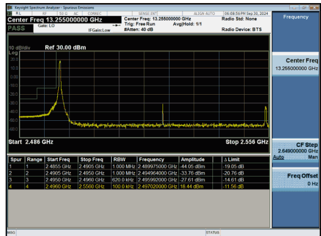
NTNV-n41-PC2-30-60-L-DFT-BPSK-Edge_1RB_Left-PASS
