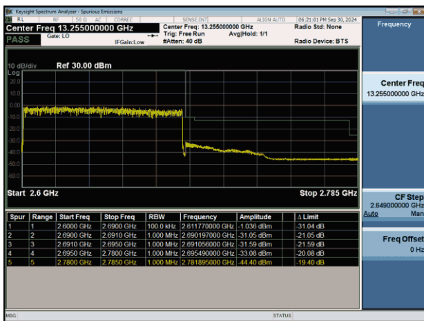
NTNV-n41-PC2-30-90-H-DFT-BPSK-Outter_Full-PASS
