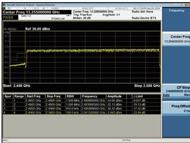
NTNV-n41-PC2-30-90-L-CP-QPSK-Outter_Full-PASS
