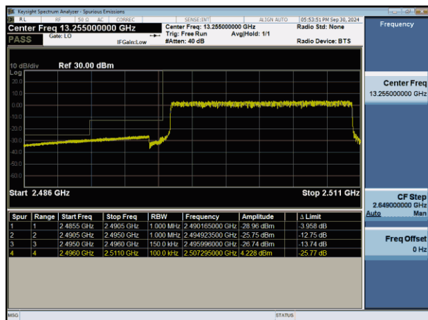
NTNV-n41-PC2-30-15-L-CP-QPSK-Outet_Full-PASS
