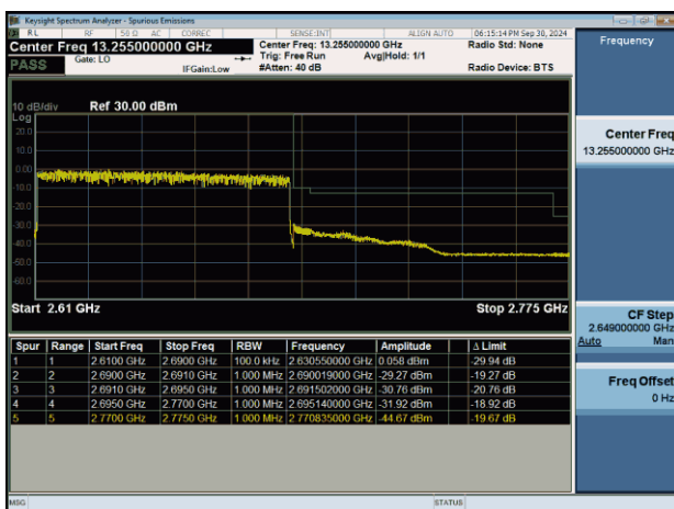
NTNV-n41-PC2-30-80-L-CP-QPSK-Outet_Full-PASS
