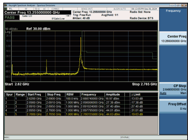
NTNV-n41-PC2-30-70-H-CP-QPSK-Edge_1RB_Right-PASS
