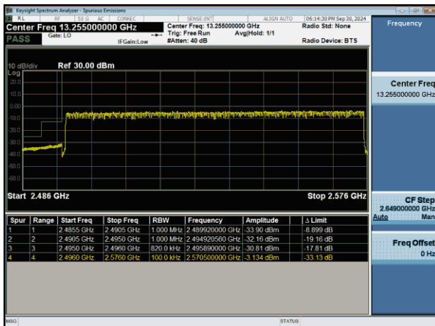
NTNV-n41-PC2-30-80-L-CP-QPSK-Outet_Full-PASS
