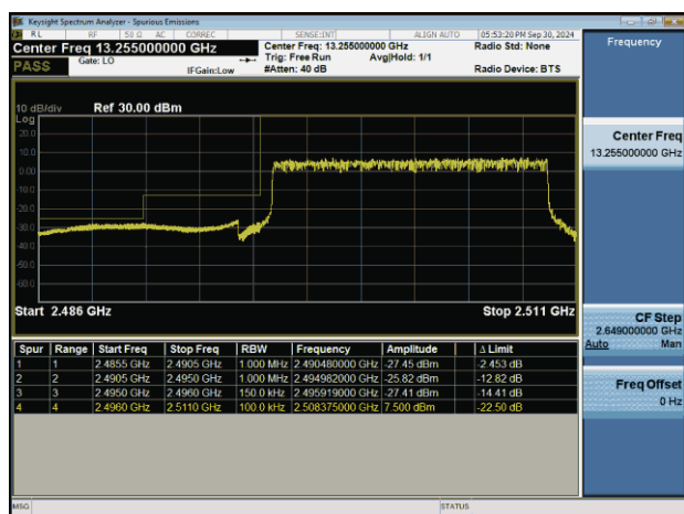
NTNV-n41-PC2-30-15-L-DFT-BPSK-Outet_Full-PASS
