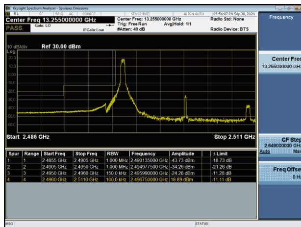
NTNV-n41-PC2-30-15-L-CP-QPSK-Edge_1RB_Left-PASS
