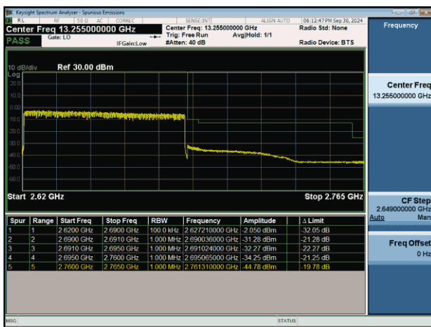
NTNV-n41-PC2-30-70-H-CP-QPSK-Outer_Full-PASS
