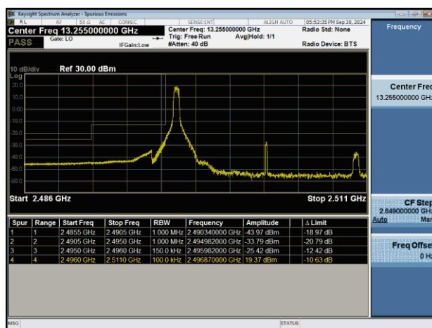
NTNV-n41-PC2-30-15-L-DFT-BPSK-Edge_1RB_Left-PASS
