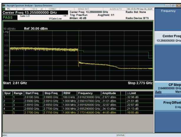
NTNV-n41-PC2-30-80-H-CP-QPSK-Outet_Full-PASS
