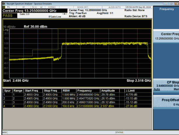
NTNV-n41-PC2-30-20-L-CP-QPSK-Outter_Full-PASS
