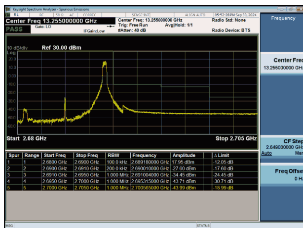
NTNV-n41-PC2-30-10-H-CP-QPSK-Edge_1RB_Right-PASS
