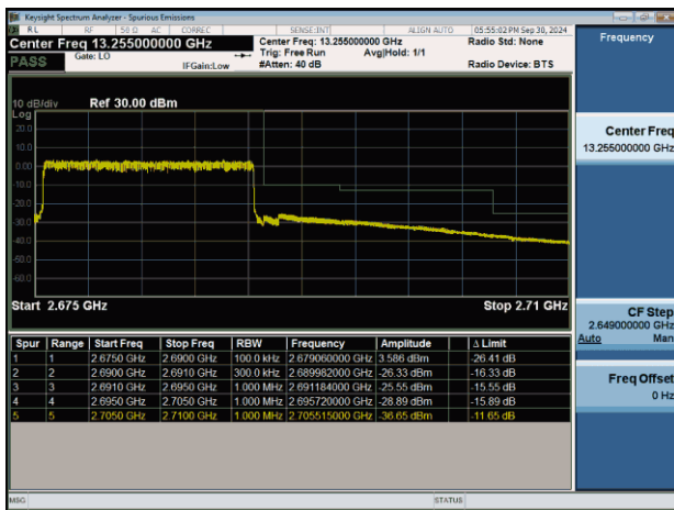
NTNV-n41-PC2-30-15-H-CP-QPSK-Outter_Full-PASS
