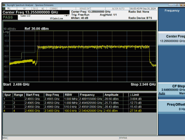
NTNV-n41-PC2-30-50-L-DFT-BPSK-Outter_Full-PASS
