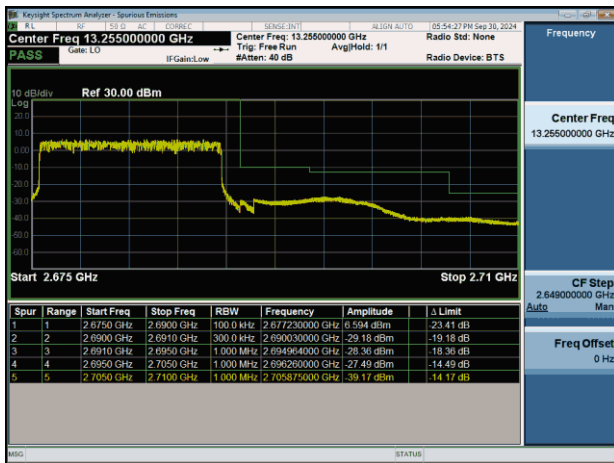
NTNV-n41-PC2-30-15-H-DFT-BPSK-Outter_Full-PASS
