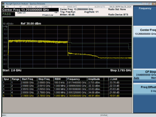
NTNV-n41-PC2-30-90-H-CP-QPSK-Outer_Full-PASS
