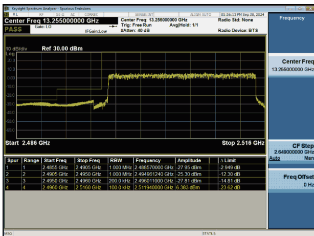
NTNV-n41-PC2-30-20-L-DFT-BPSK-Outter_Full-PASS
