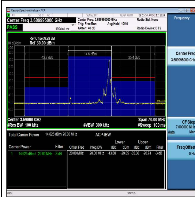
NTNV_N48_PC3_30_20_H_TID3_#1_-20_20
