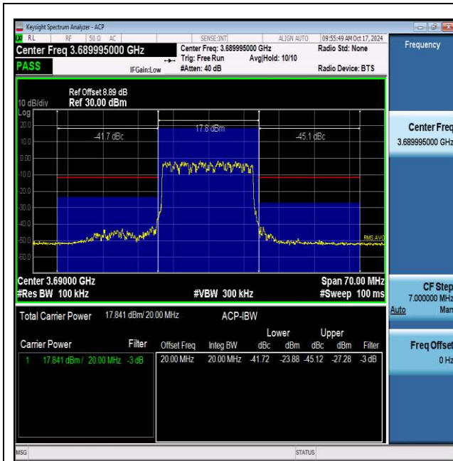
NTNV_N48_PC3_30_20_H_TID1_#1_-20_20
