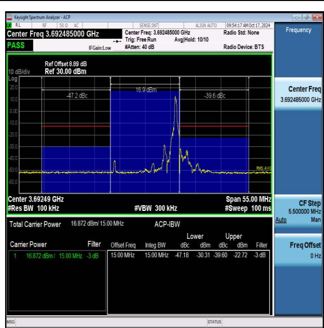
NTNV_N48_PC3_30_15_H_TID3_#1_+15_15
