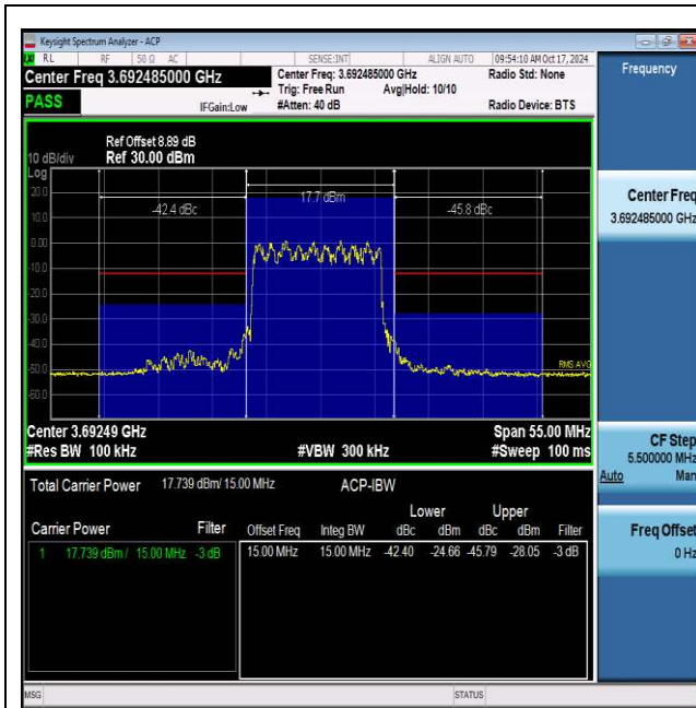
NTNV_N48_PC3_30_15_H_TID1_#1_-15_15
