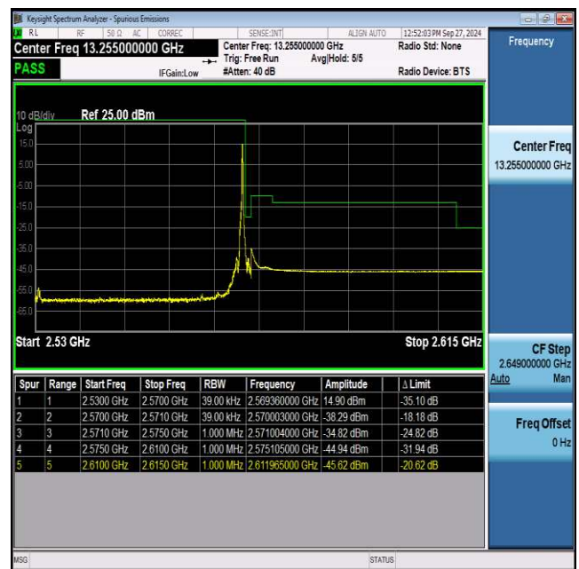
NTNV_N7_PC3_15_40_H_TID18_#1
