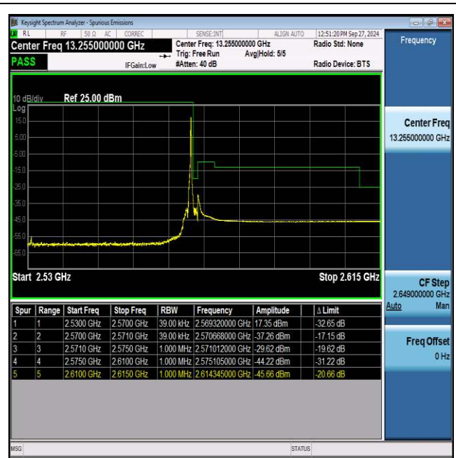
NTNV_N7_PC3_15_40_H_TID3_#1
