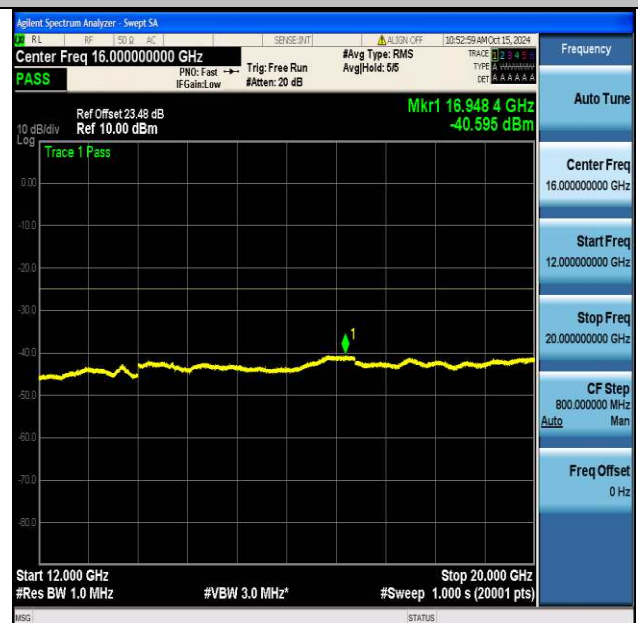
NTNV_N7_PC3_15_40_H_TID1_NS_01_12000_20000_#1
