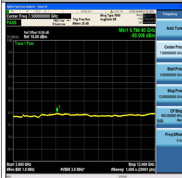
NTNV_N7_PC3_15_40_H_TID1_NS_01_3000_12000_#1
