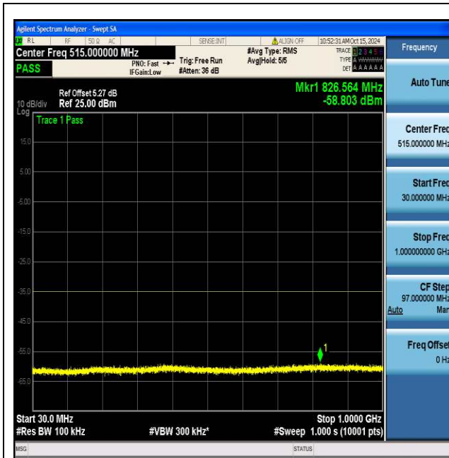
NTNV_N7_PC3_15_40_H_TID1_NS_01_30_1000_#1
