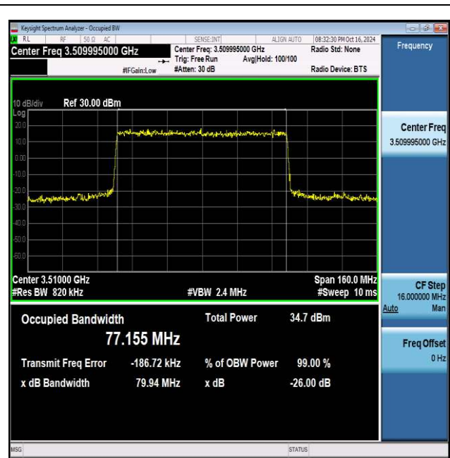
NTNV_N77-3450-3550_PC2_30_80_H_TID2_Ant1#1
