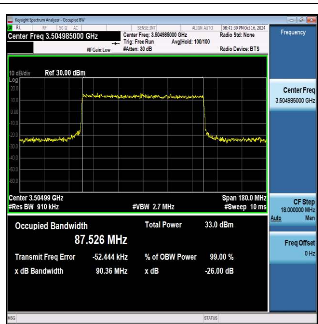
NTNV_N77-3450-3550_PC2_30_90_H_TID6_Ant1#1
