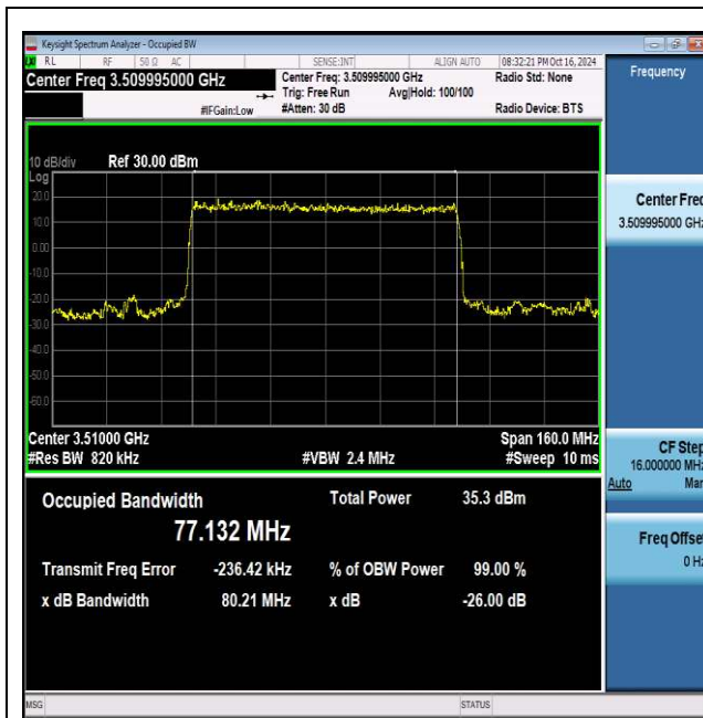
NTNV_N77-3450-3550_PC2_30_80_H_TID1_Ant1#1
