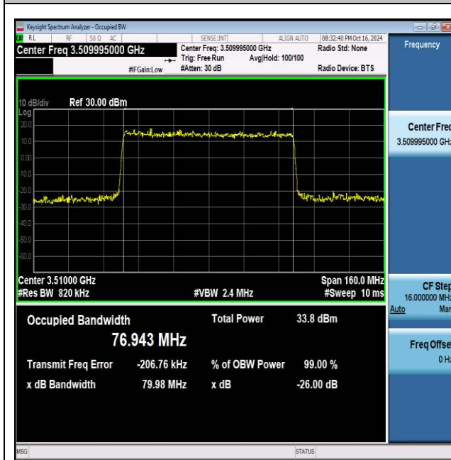
NTNV_N77-3450-3550_PC2_30_80_H_TID3_Ant1#1
