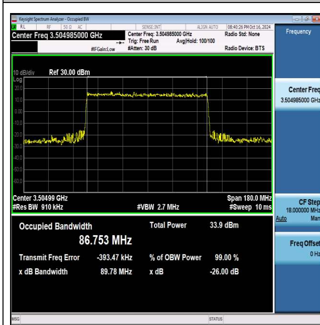
NTNV_N77-3450-3550_PC2_30_90_H_TID3_Ant1#1
