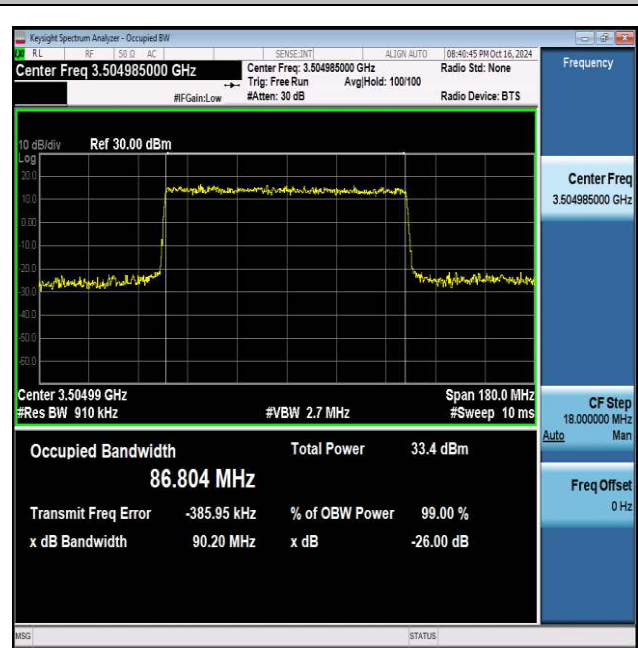
NTNV_N77-3450-3550_PC2_30_90_H_TID4_Ant1#1
