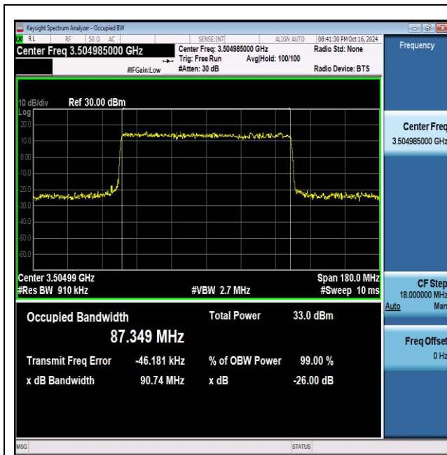
NTNV_N77-3450-3550_PC2_30_90_H_TID5_Ant1#1
