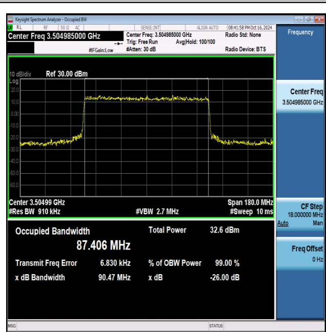
NTNV_N77-3450-3550_PC2_30_90_H_TID8_Ant1#1
