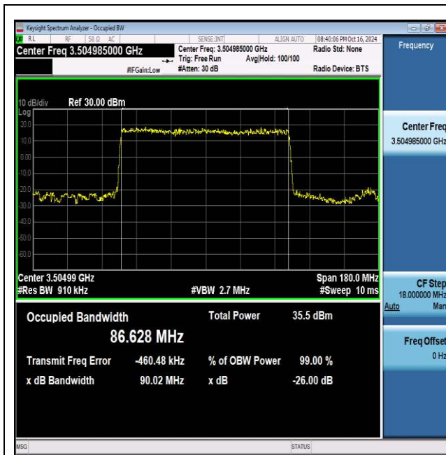
NTNV_N77-3450-3550_PC2_30_90_H_TID1_Ant1#1
