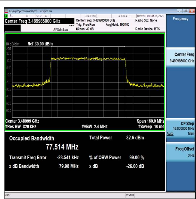
NTNV_N77-3450-3550_PC2_30_80_L_TID8_Ant1#1
