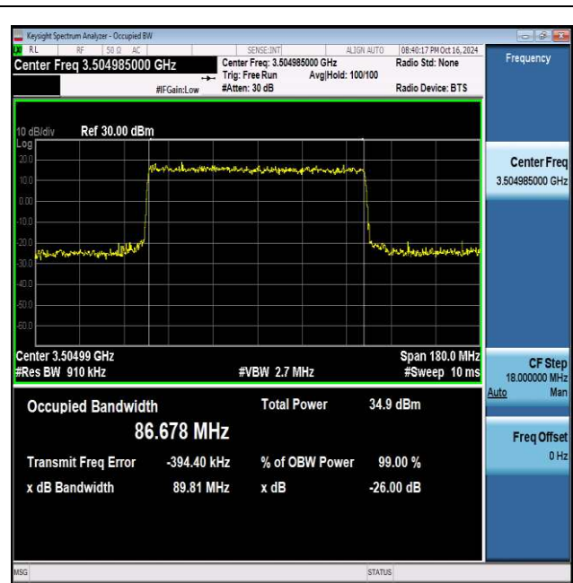
NTNV_N77-3450-3550_PC2_30_90_H_TID2_Ant1#1
