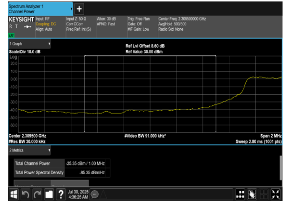
N30(5M)_DFT-s- OFDM_BPSK_Outer_Full_High_CH_CHP_PASS
