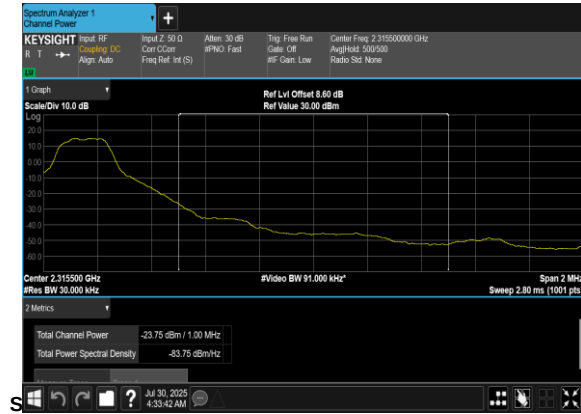
N30(5M)_DFT-s- OFDM_QPSK_Edge_1RB_Right_High_CH_CHP_PAS
