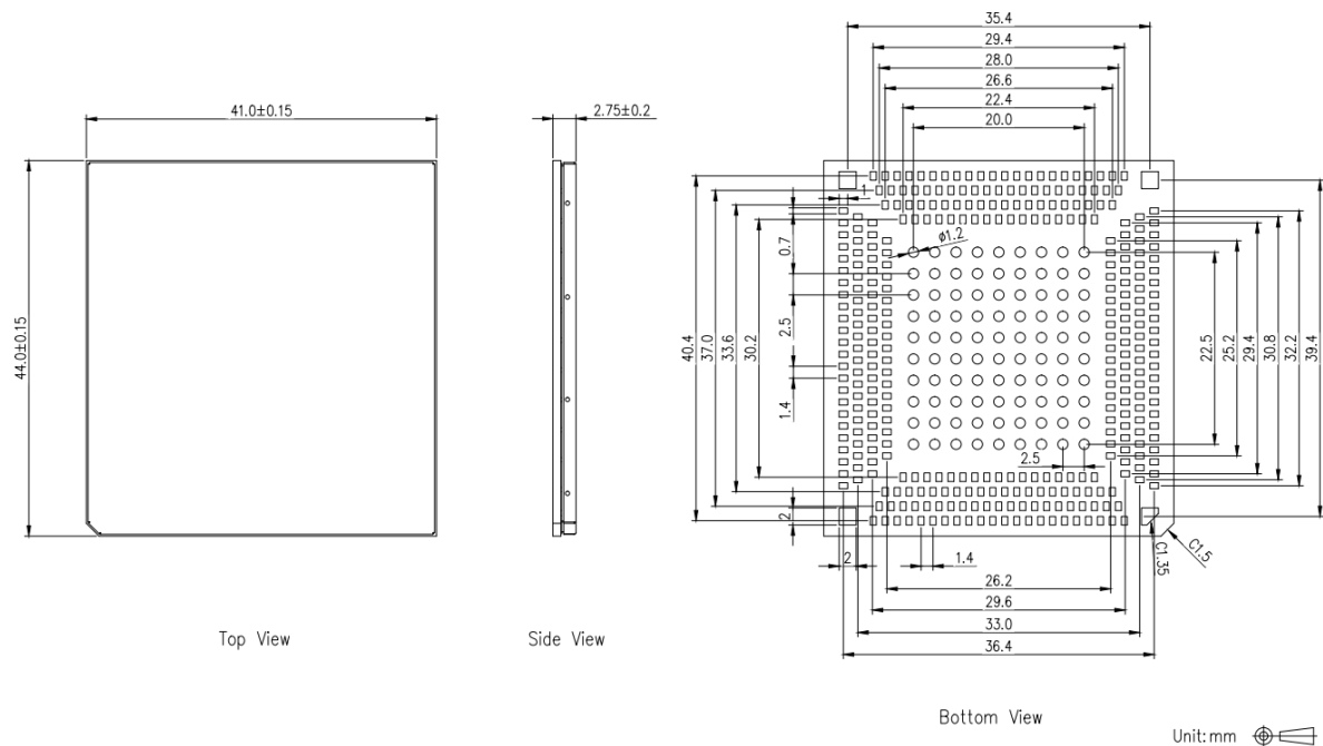
Figure 4-2 Structure size chart
