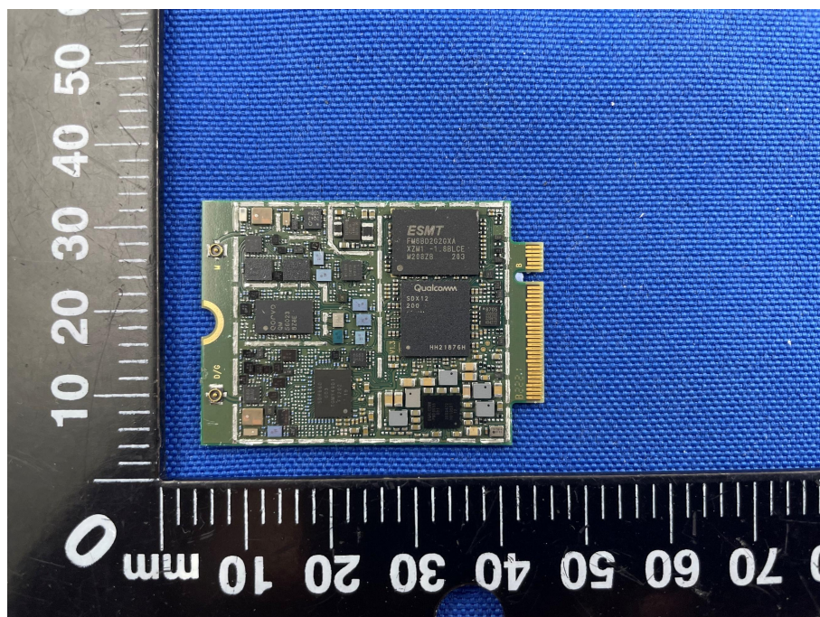
RF MODULE TOP VIEW-FM101-GL (WITHOUT SHIELDING)
