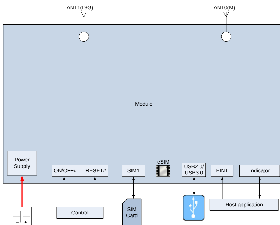
Figure 1. Application block
