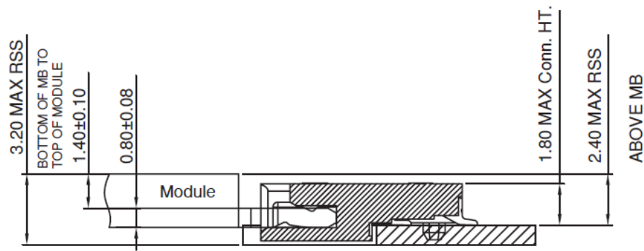
Figure 32. Stack-up mid-mount single-sided module
