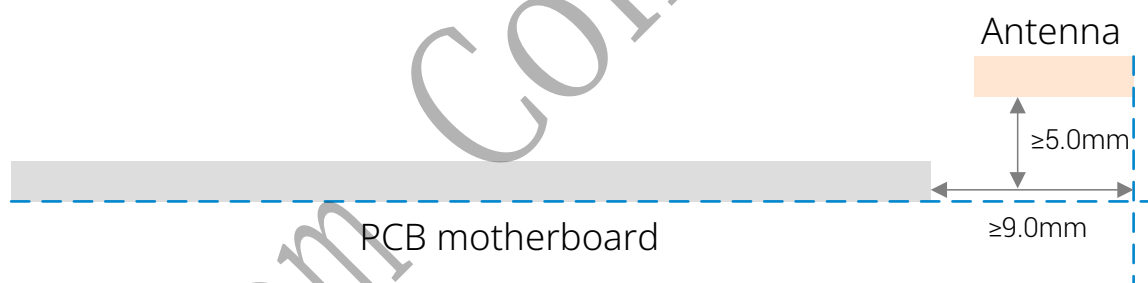
Figure 28. Antenna location
