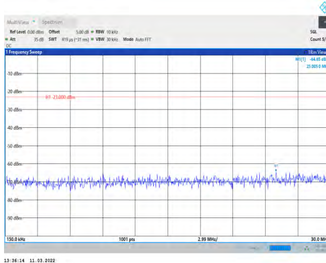
Band5-10MHz-QPSK-20450-1RB#0-Range2:0.15~30MHz
