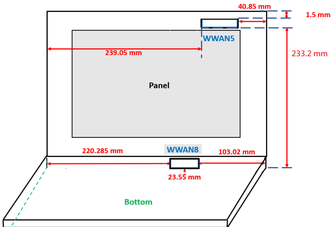
Photograph 5. Antenna position of EUT
