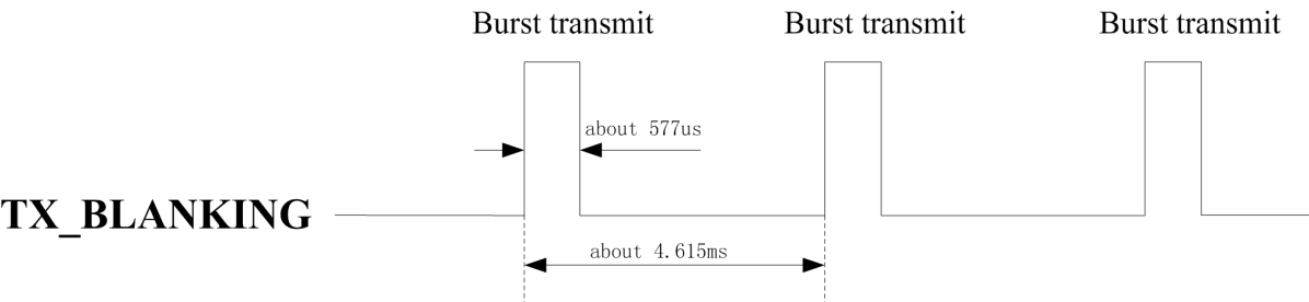
Figure 3-17 TX_BLANKING Timing
