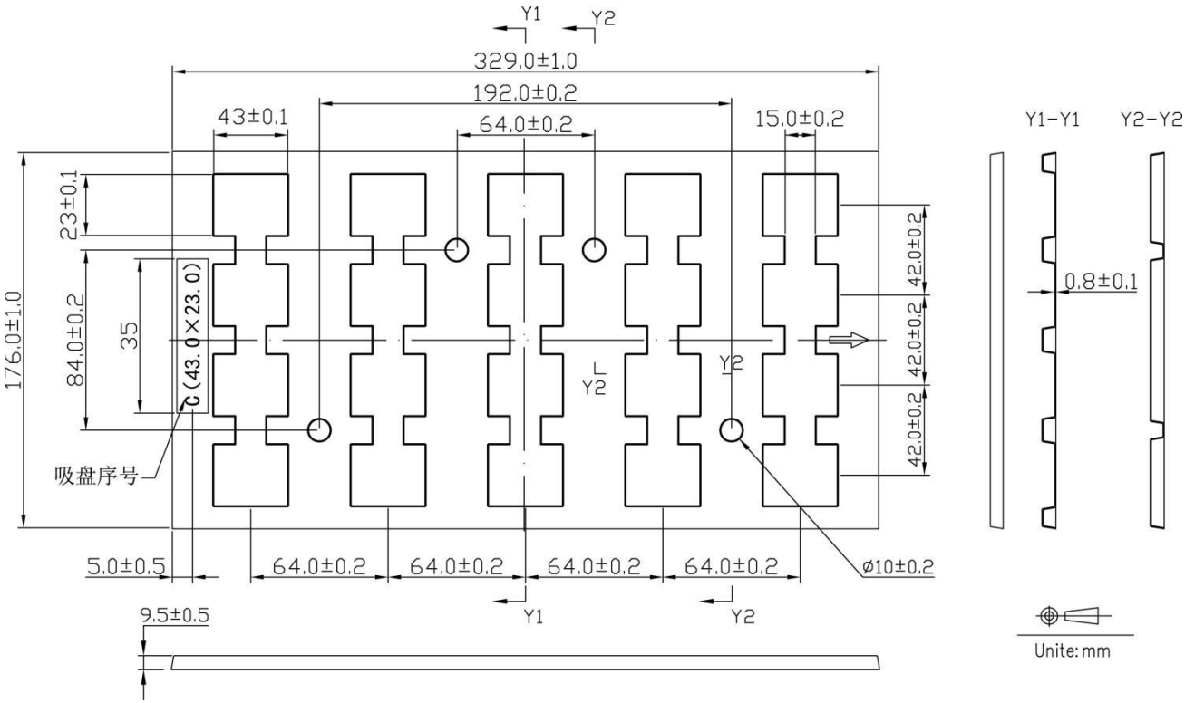
Figure 5-5 Tray Size
