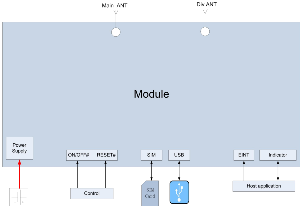
Figure 2-1 Application Framework
