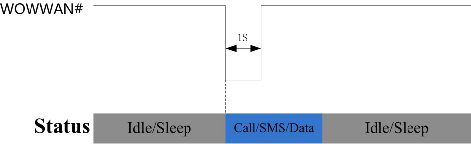
Figure 3-16 WOWWAN# Timing
