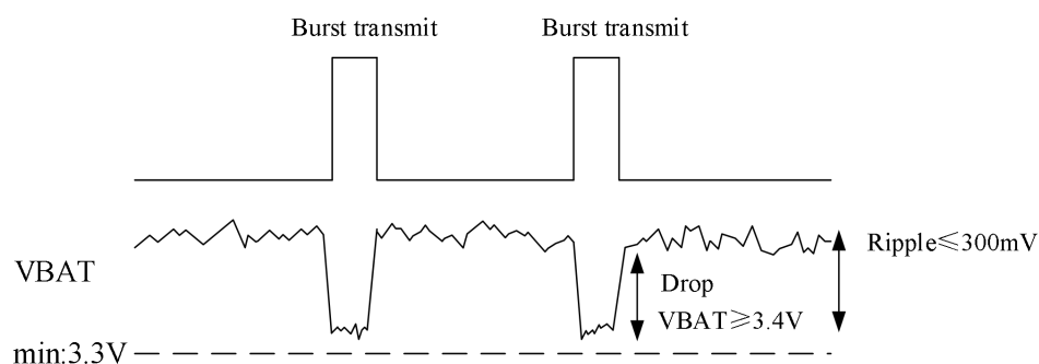
Figure 3-3 Power Limit
