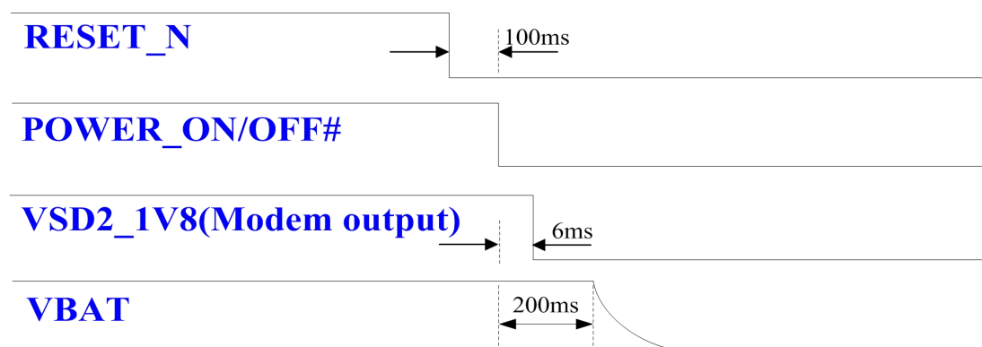
Figure 5-3 Power off Timing Sequence Diagram
