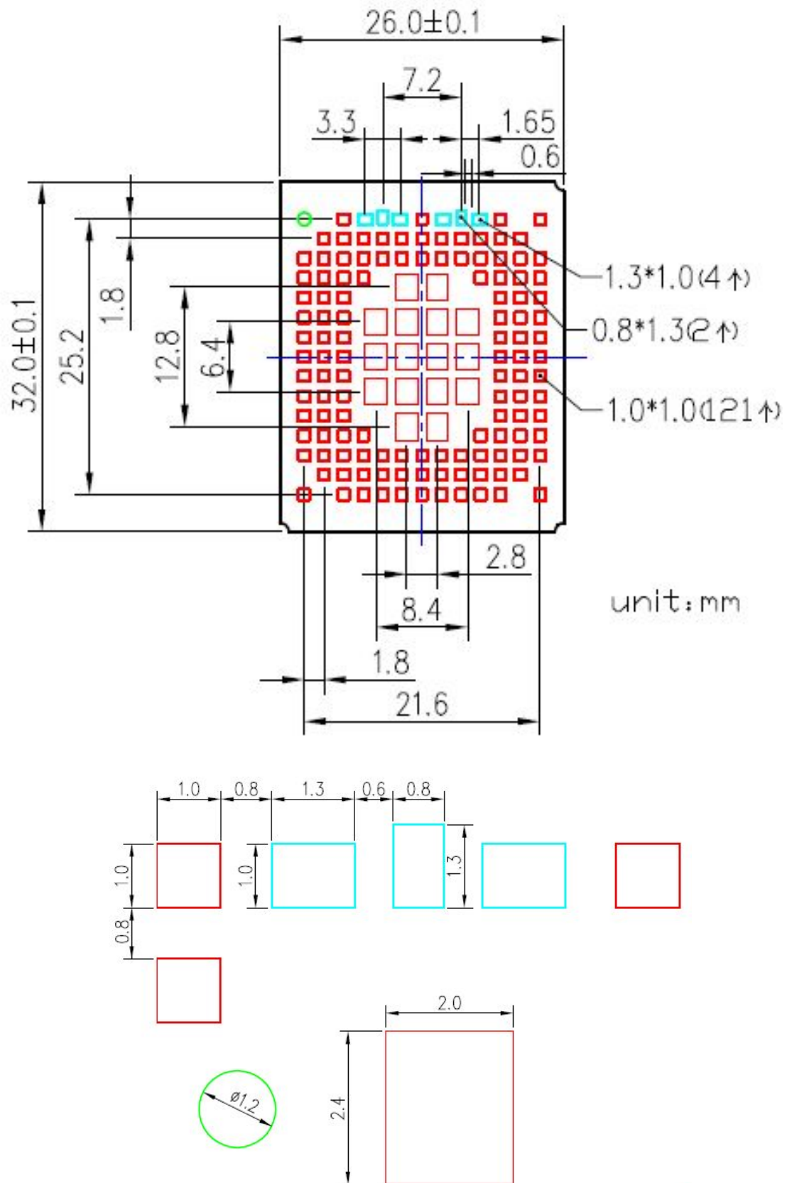
Figure 3-3 Structure Diagram of PCB Layout
